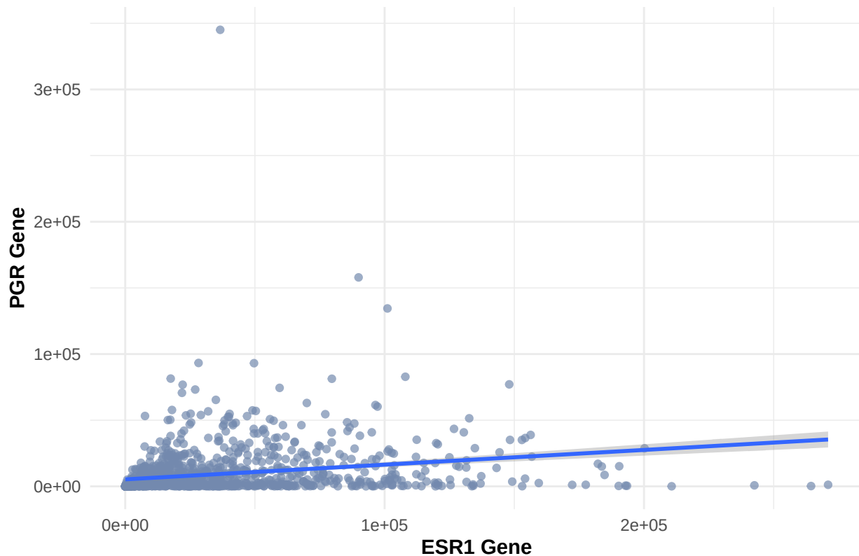
ESR1 Gene vs. PGR Gene Scatterplot
