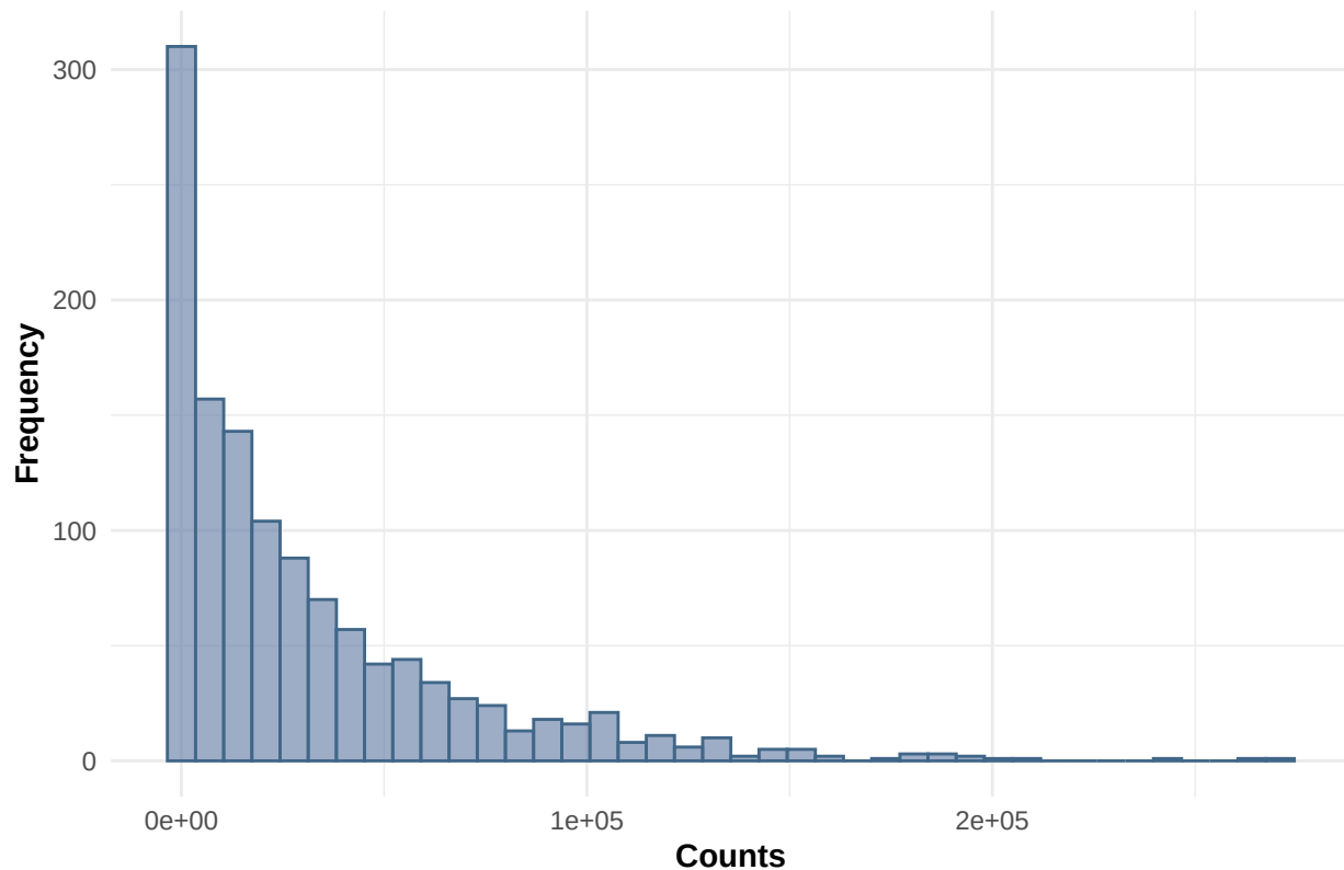
Histogram of Counts for Gene ESR1
