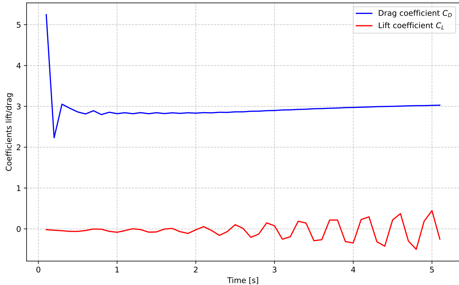
Flow around cylinder ( Re = 100.0 ) with DDN
