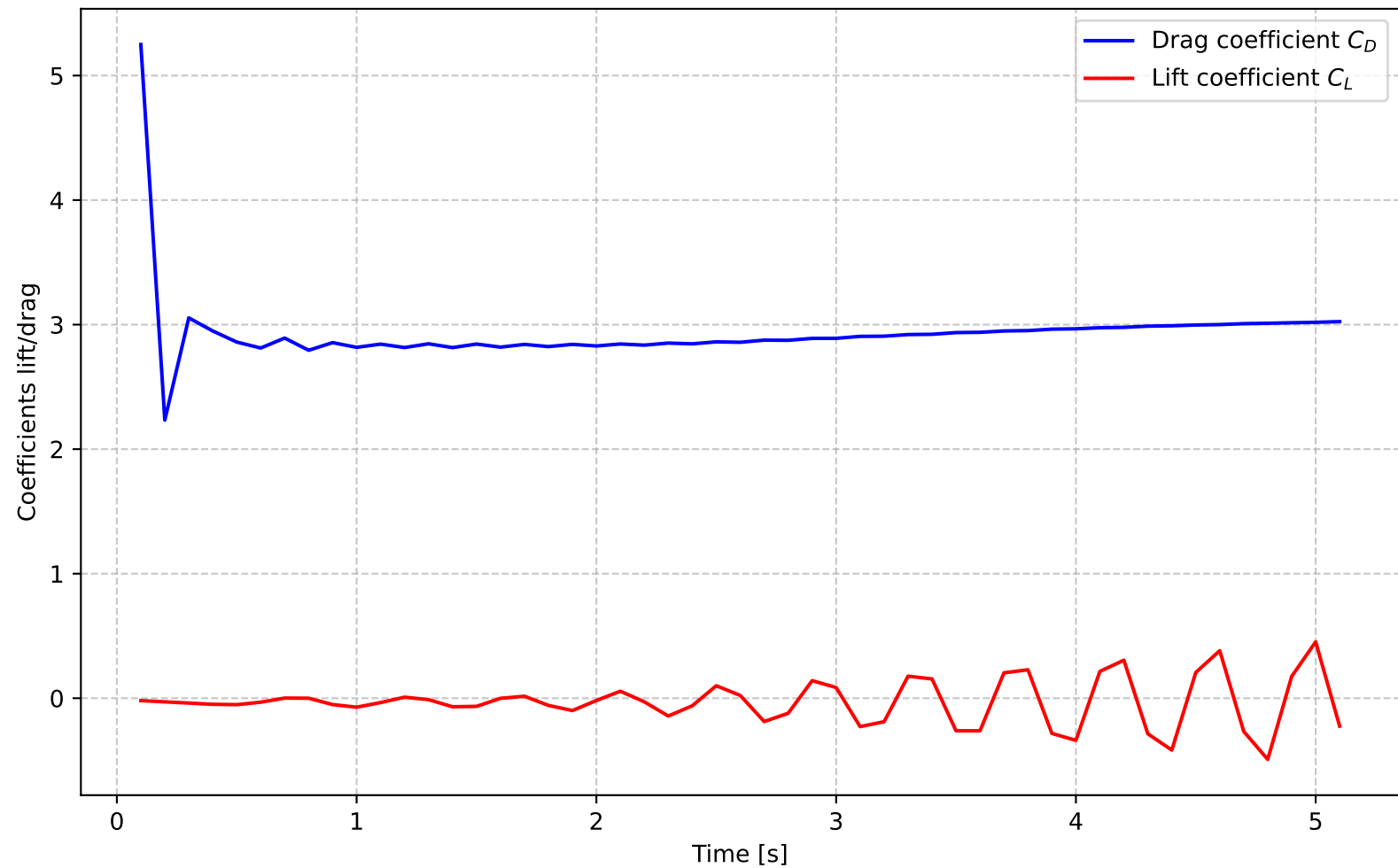
Flow around cylinder ( Re = Re )
