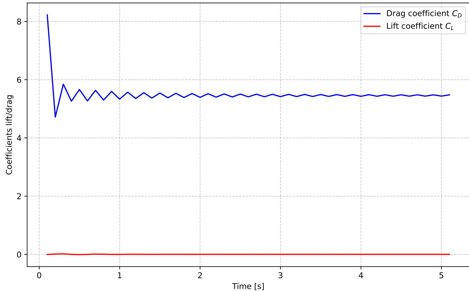
Flow around cylinder ( Re = 20.0 )
