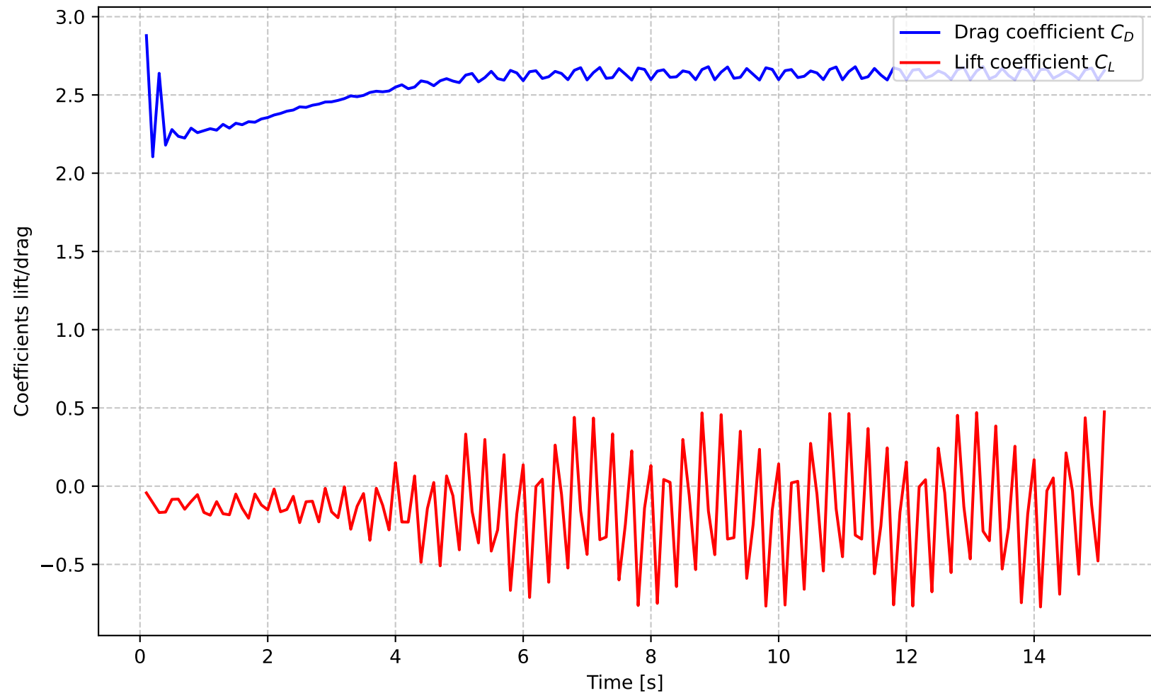
Flow around cylinder ( Re = 200.0 ) mix, change U
