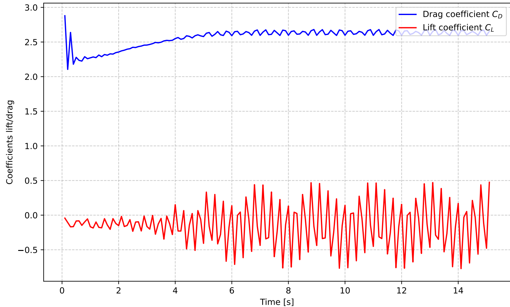
Flow around cylinder ( Re = 200.0 ) orig, change U
