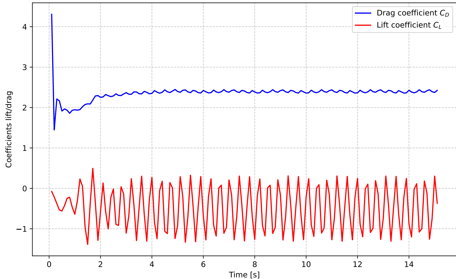
Flow around cylinder ( Re = 320.0 ) with DDN
