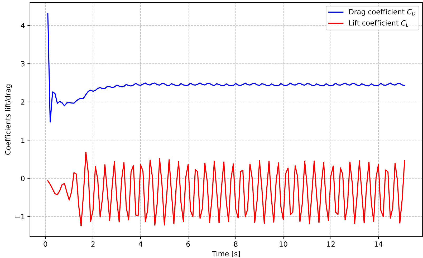
Flow around cylinder ( Re = 320.0 ) with D(u)
