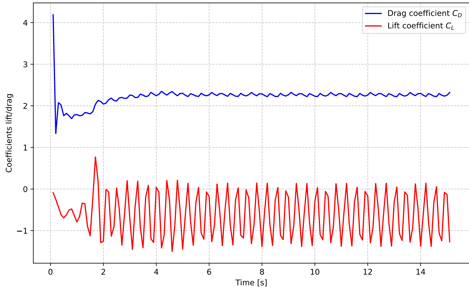
Flow around cylinder ( Re = 400.0 ) with DDN
