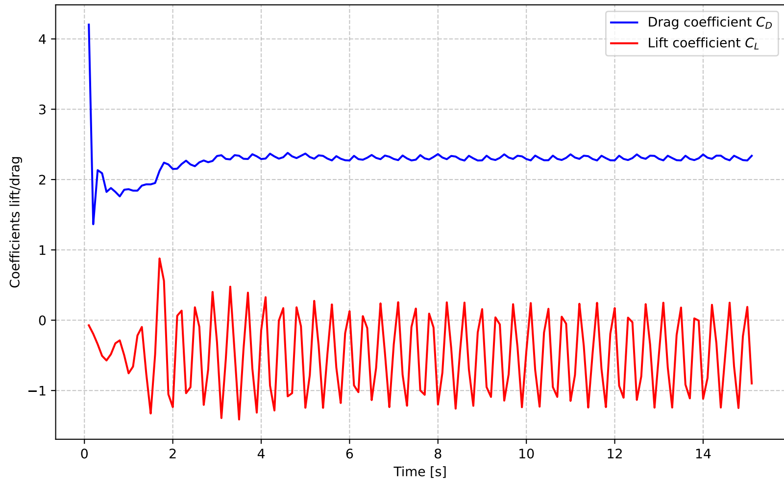
Flow around cylinder ( Re = 400.0 ) with D(u)
