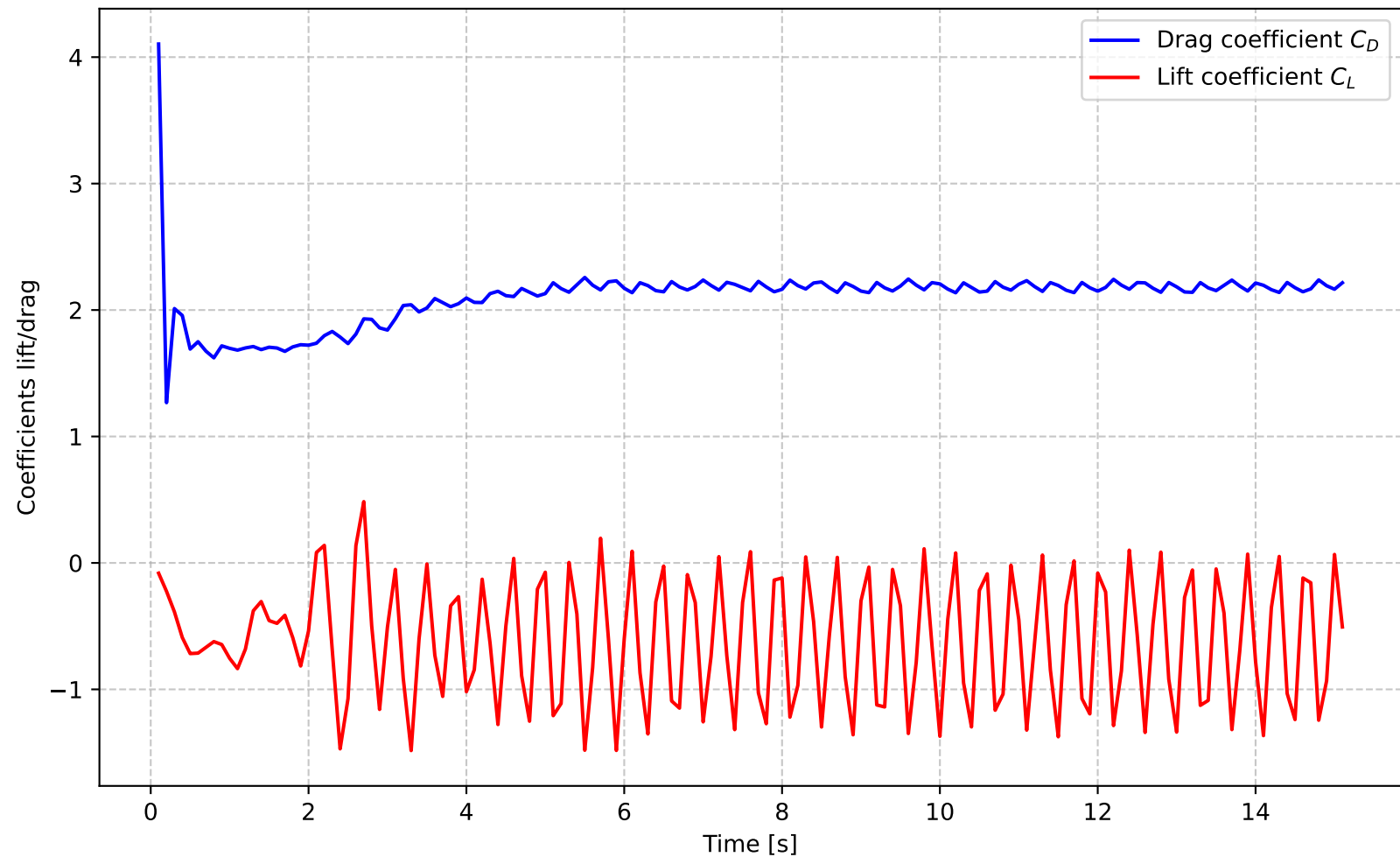
Flow around cylinder ( Re = 500.0 ) with D(u)
