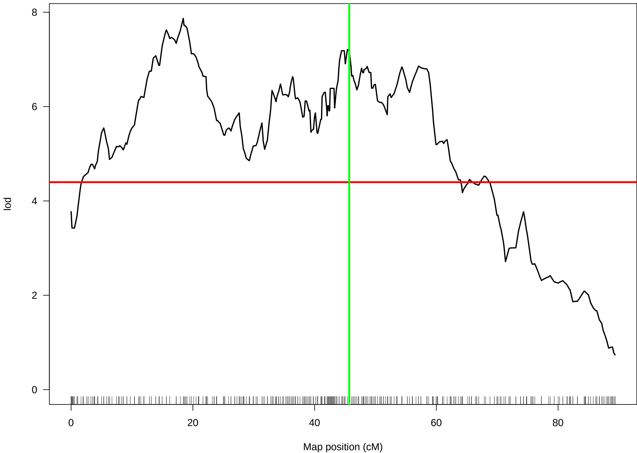
COL – Chr6 (alpha=0.05)
