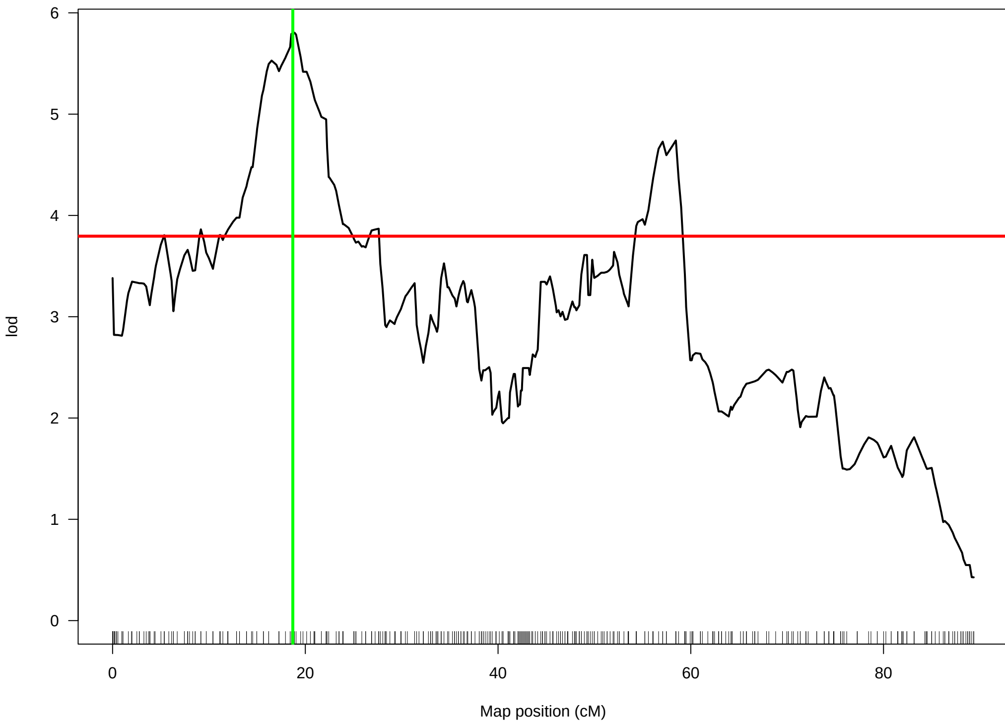
COLL – Chr6 (alpha=0.05)
