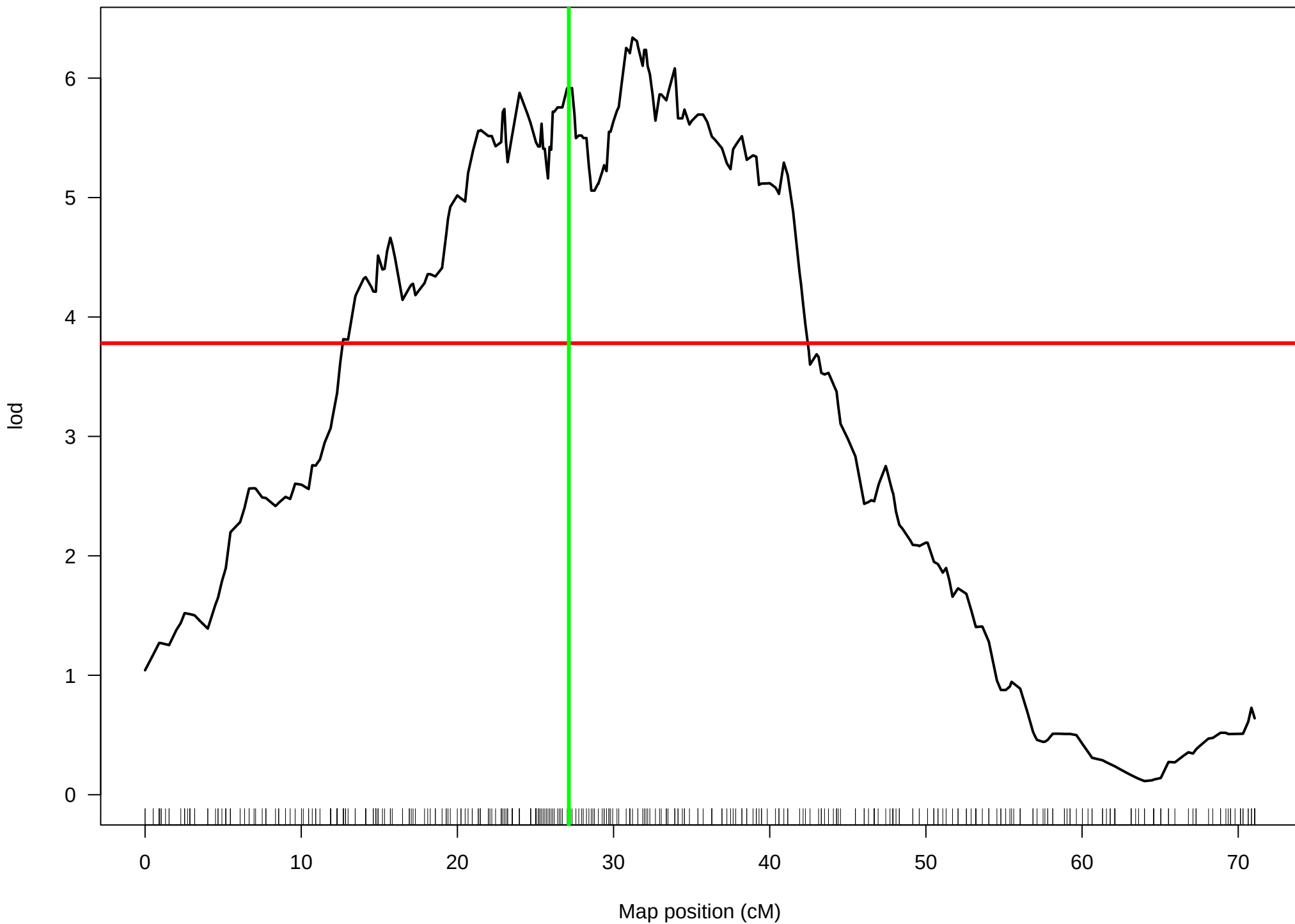
LABW – Chr5 (alpha=0.05)
