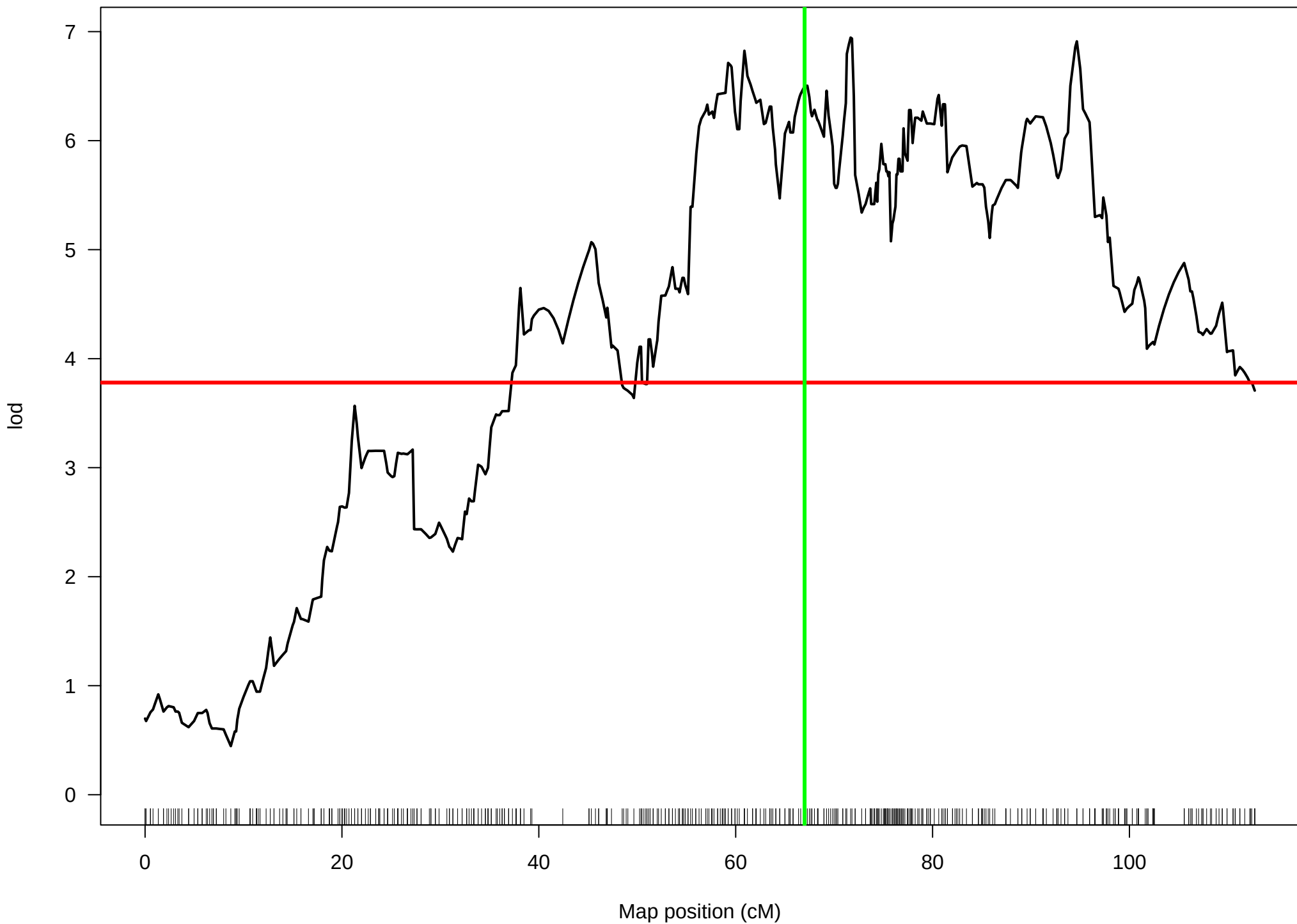
LABW – Chr2 (alpha=0.05)
