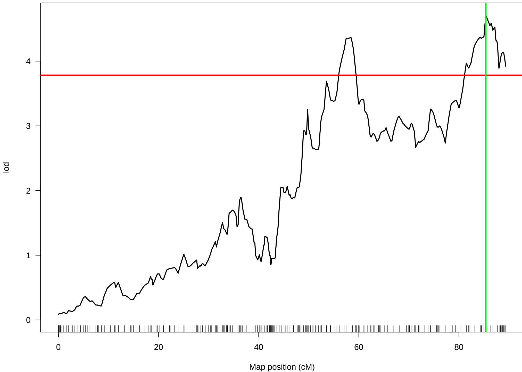
LABW – Chr6 (alpha=0.05)
