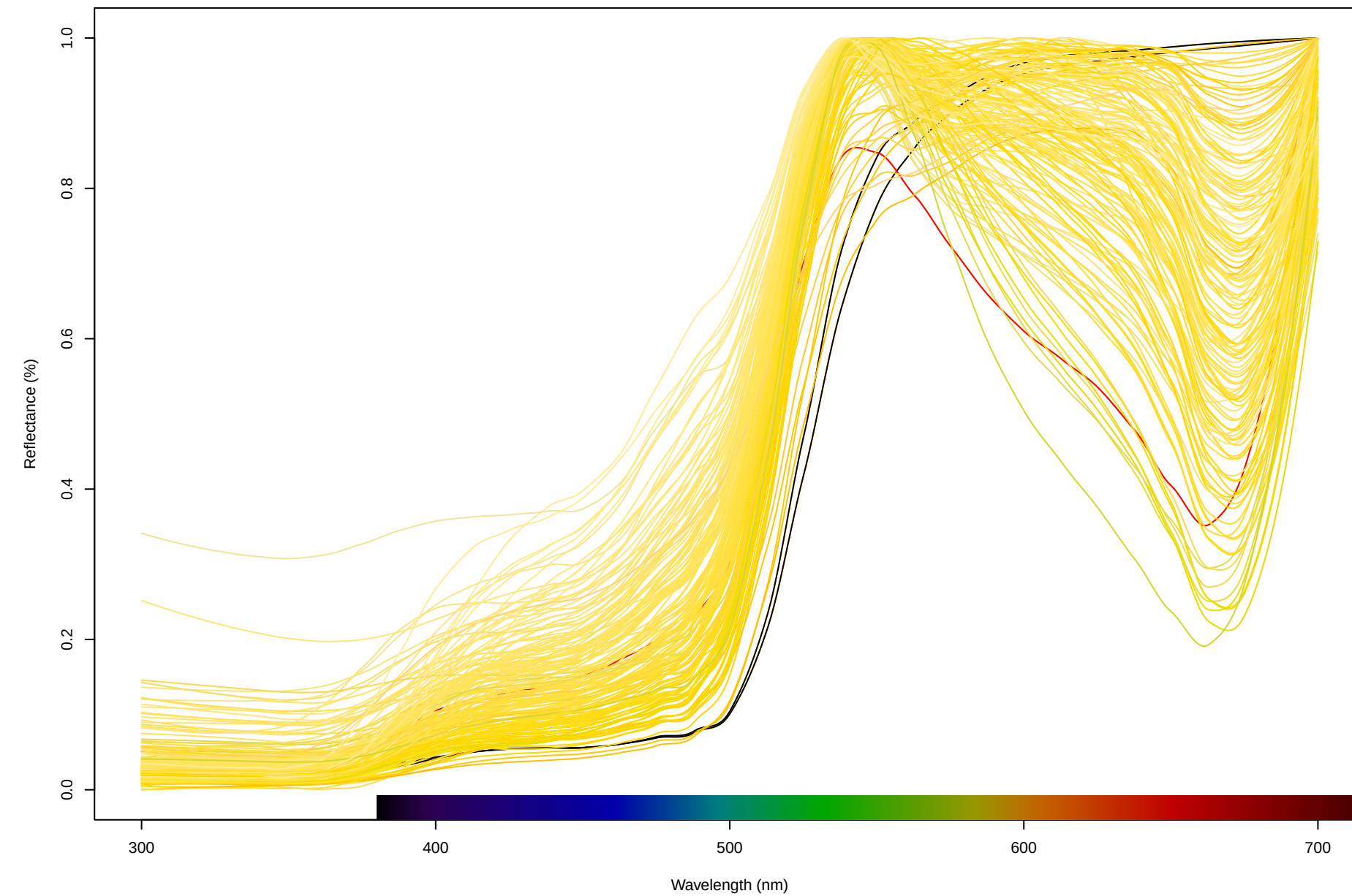
Bract Spectra
