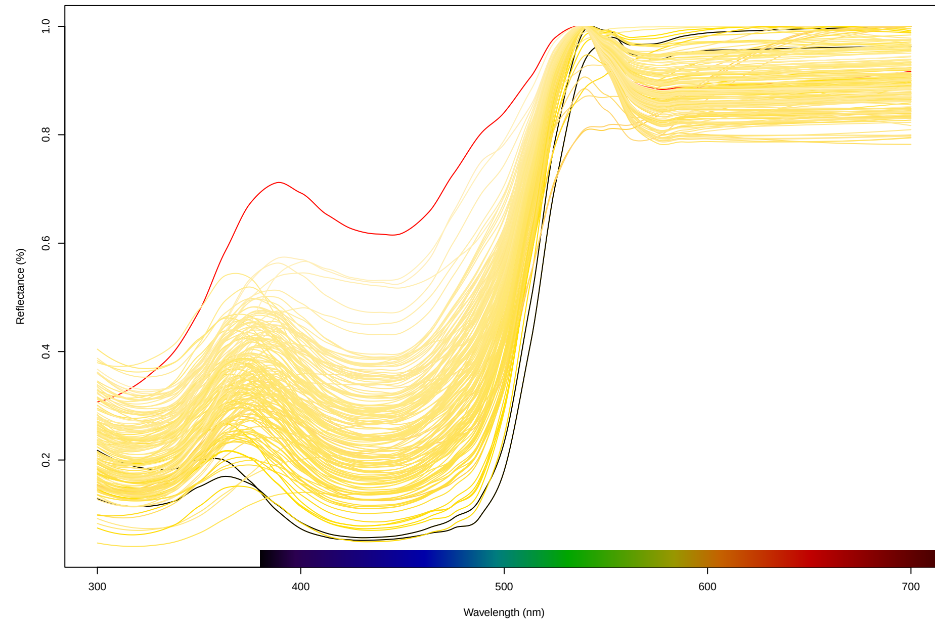
Labellum Spectra
