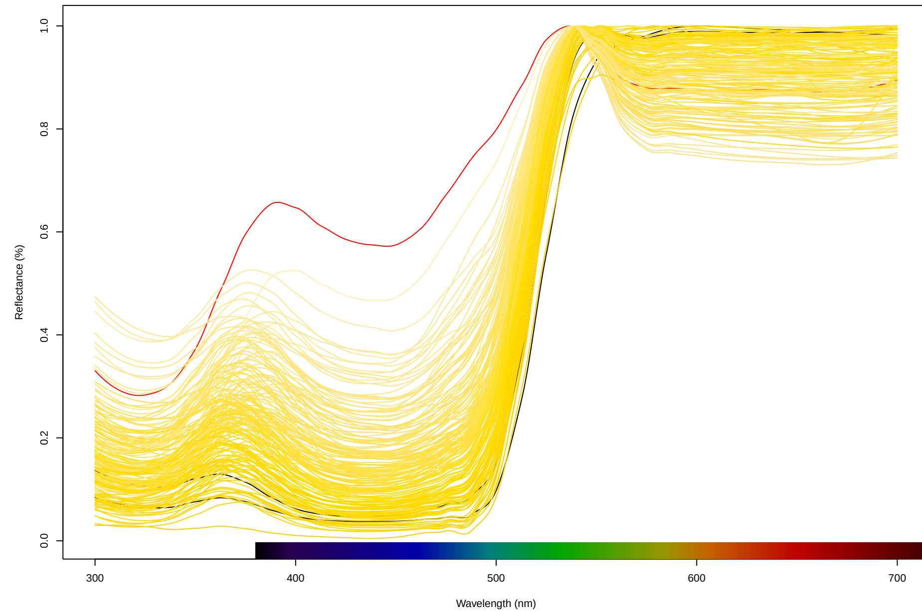
Petal Spectra
