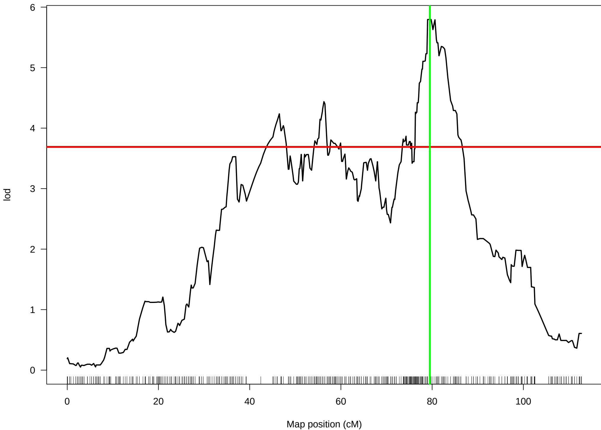
EFNSC40 – Chr2 (alpha=0.05)
