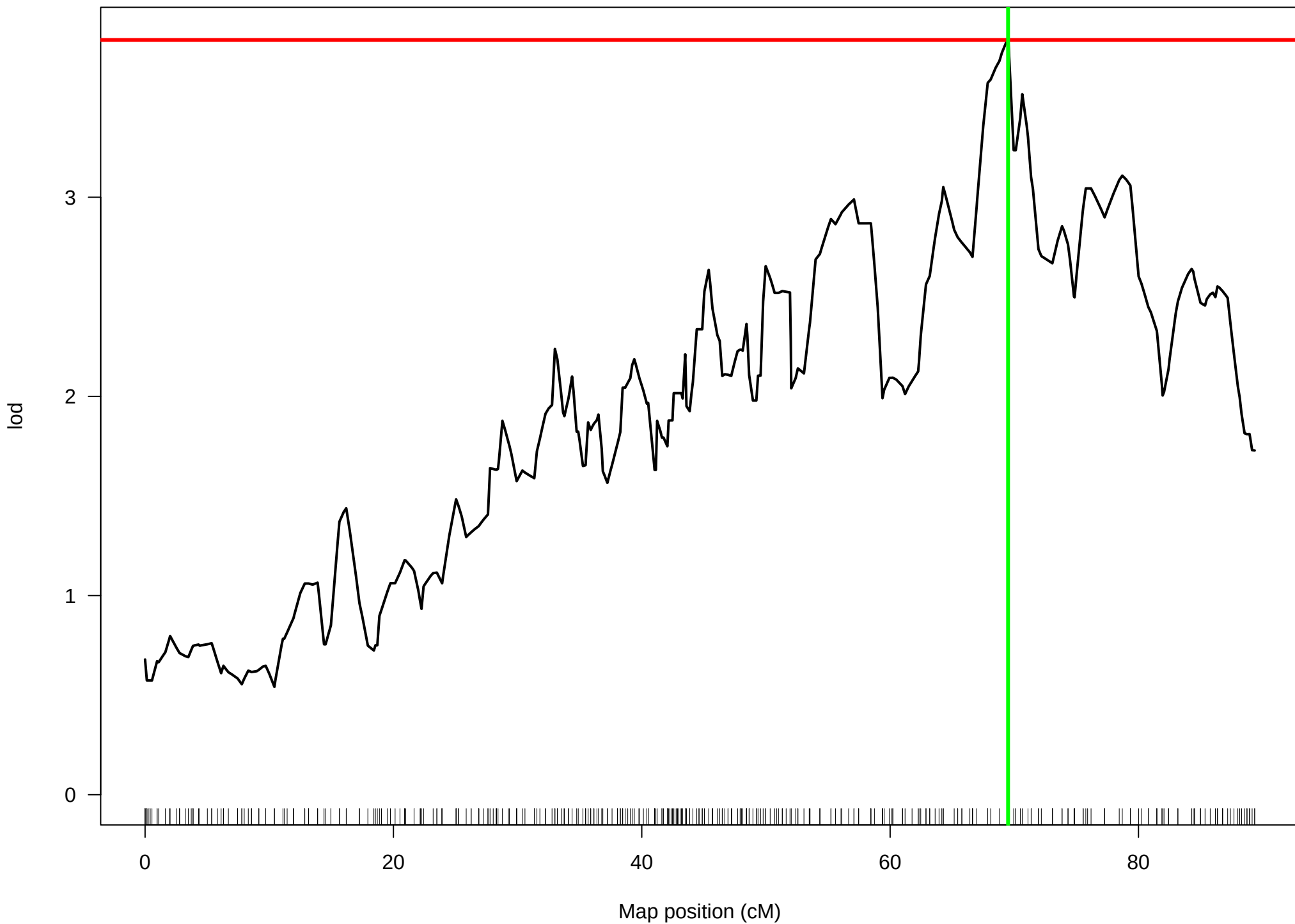
TUA – Chr6 (alpha=0.05)
