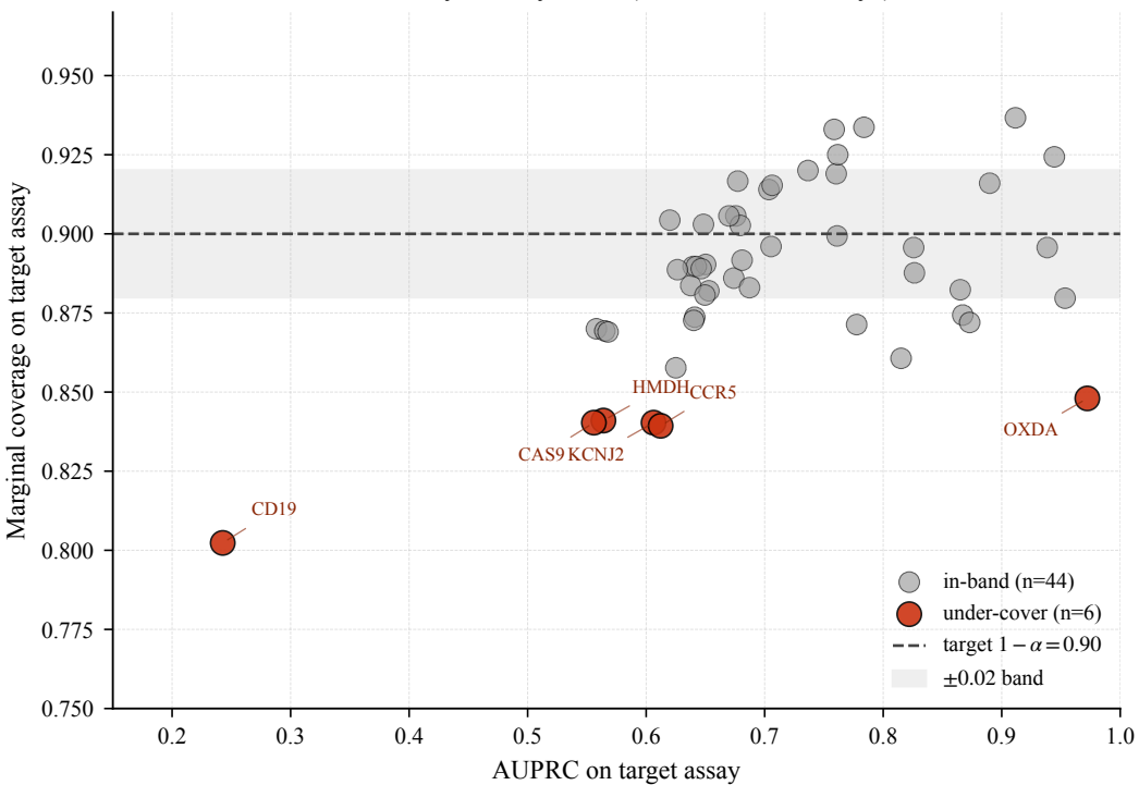
ProteinGym assay-LOO (n=50 held-out assays)
