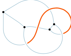
Figure 1: over-over path example
