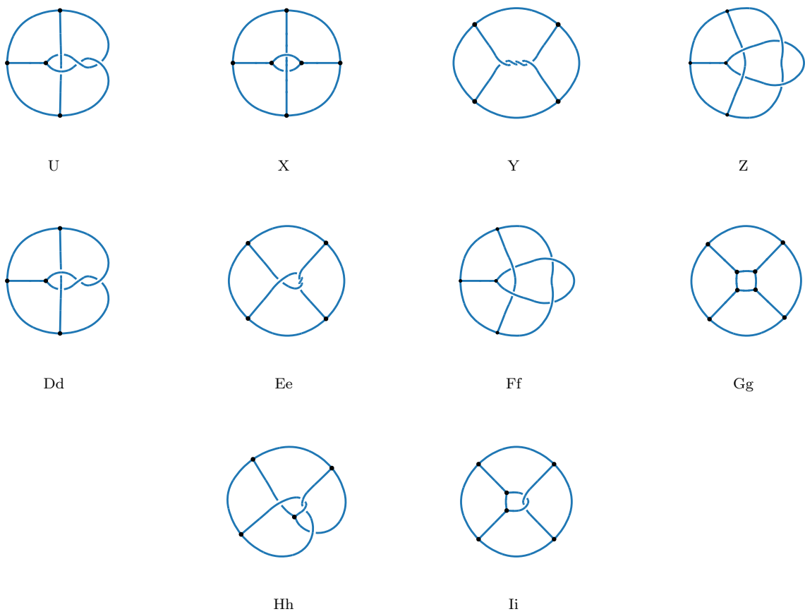
Figure 2: Bonded knots. Each entry is represented by two rows: the diagram and its label.
