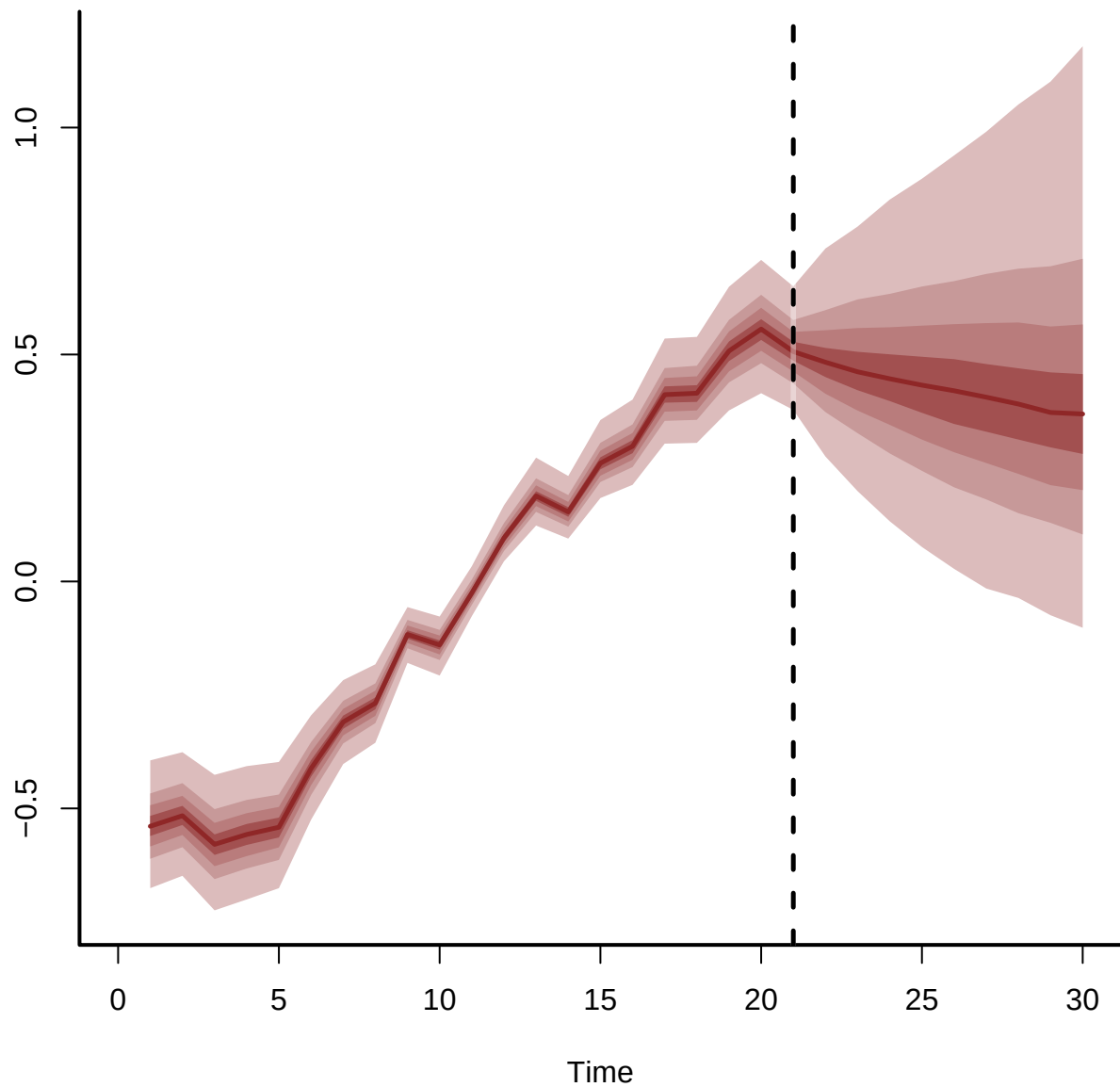
Estimated trend for series_22
