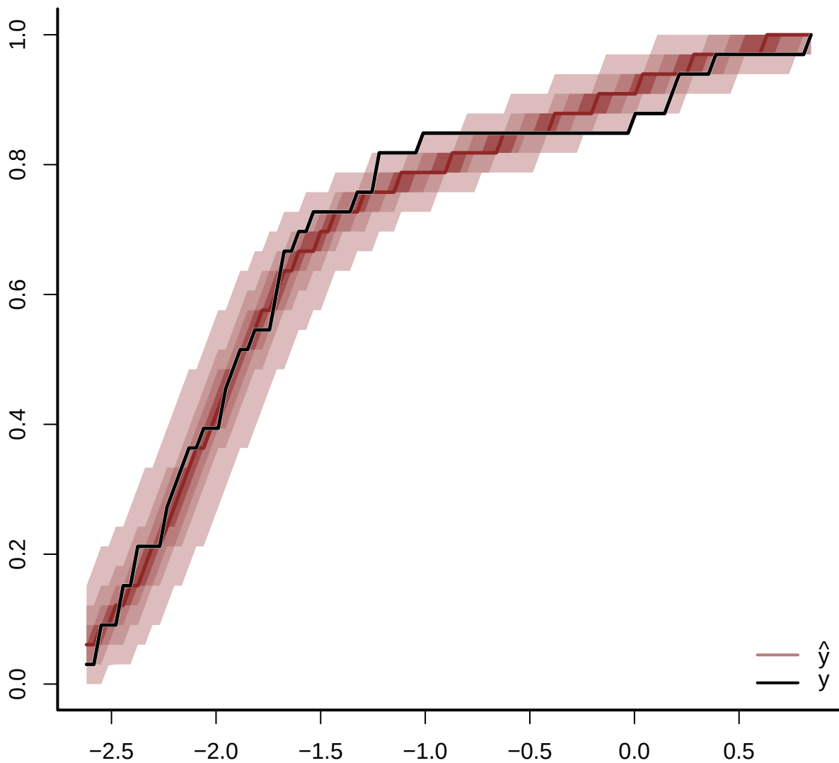
Predictive CDF for RAJA_SPINICAUDA
