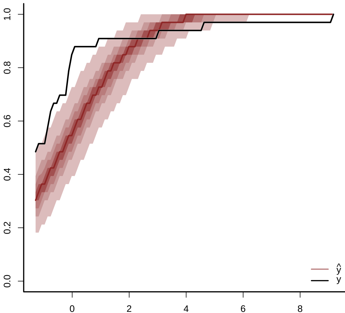
Predictive CDF for UROPHYCIS_TENUS
