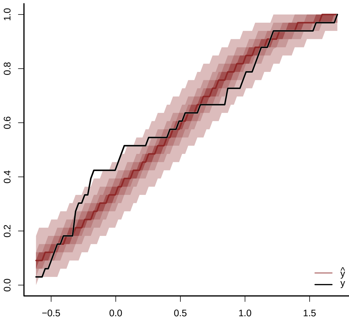
Predictive CDF for NEZUMIA_BAIRDI
