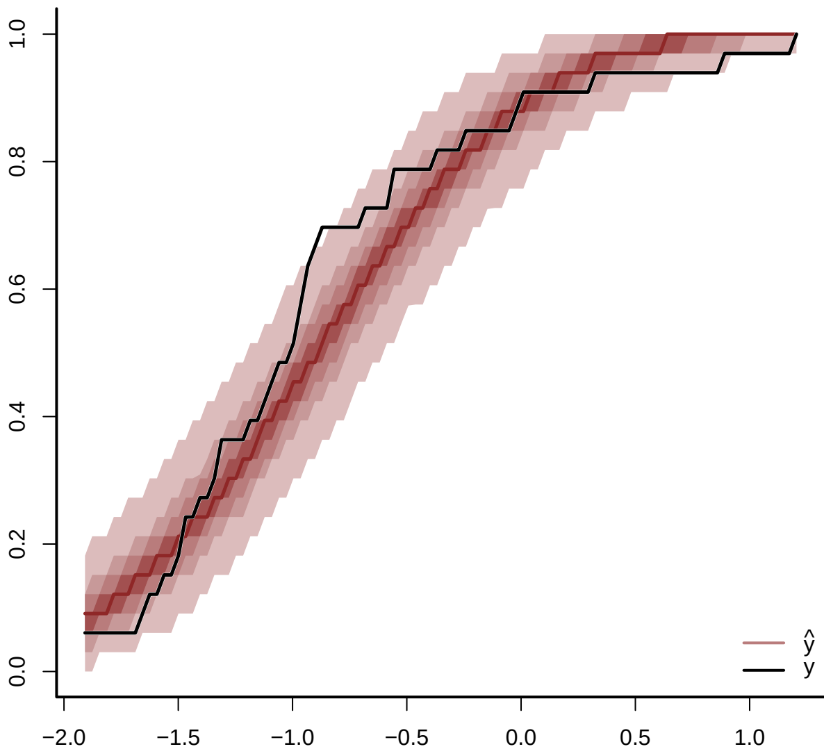
Predictive CDF for LYCODES_VAHLII
