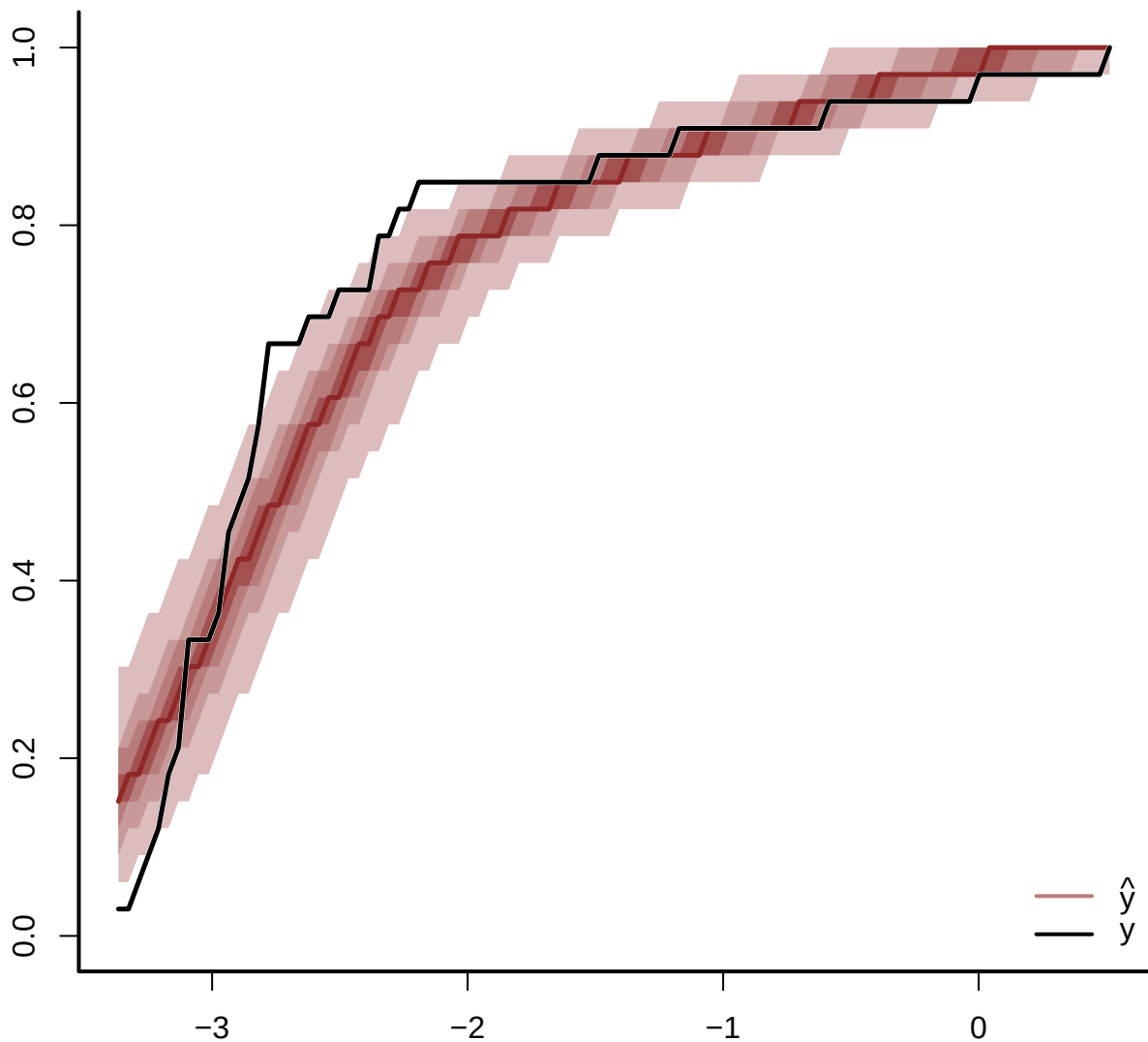
Predictive CDF for LYCODES_ESMARKI
