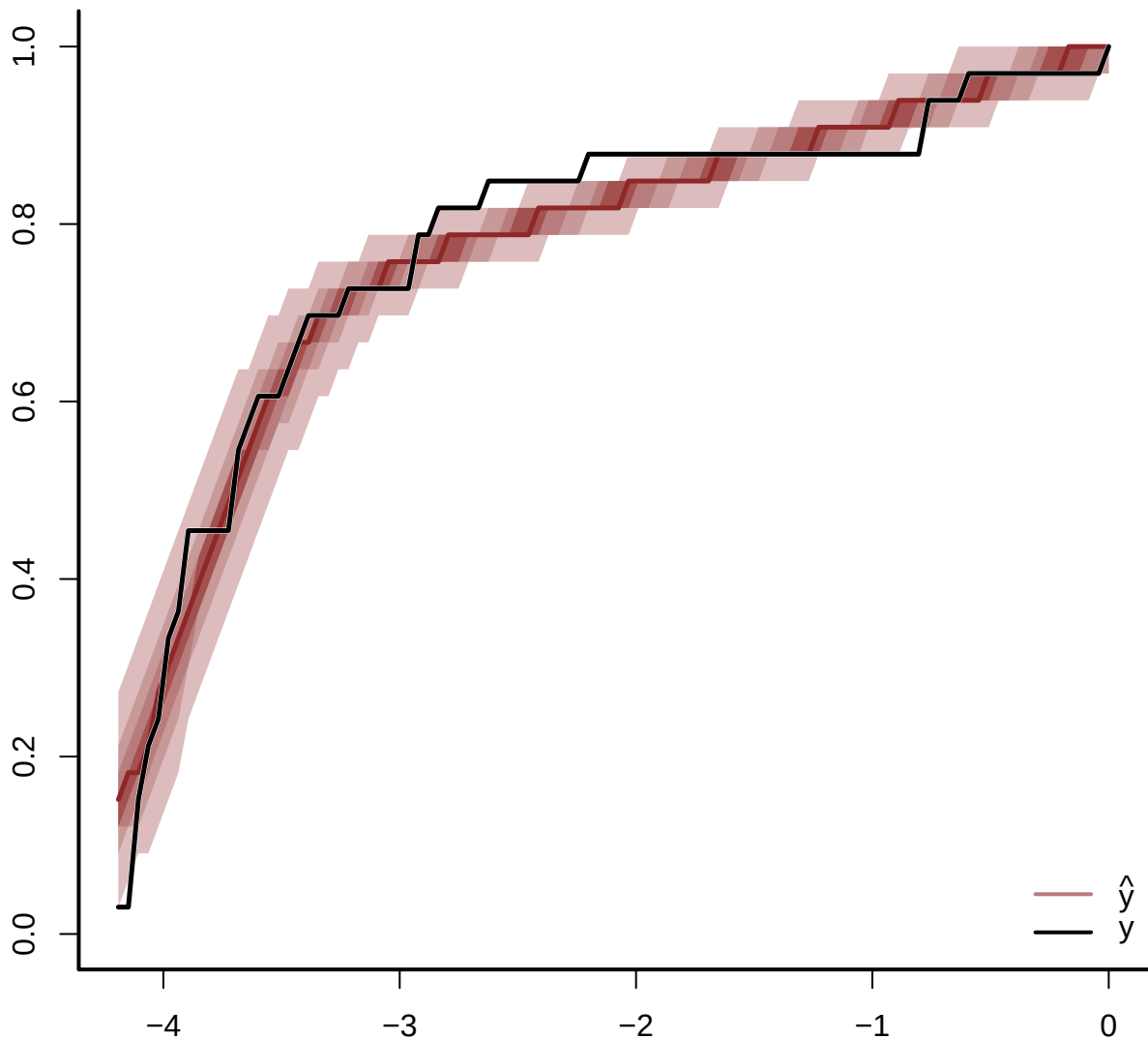
Predictive CDF for ANARHICHAS_LUPUS
