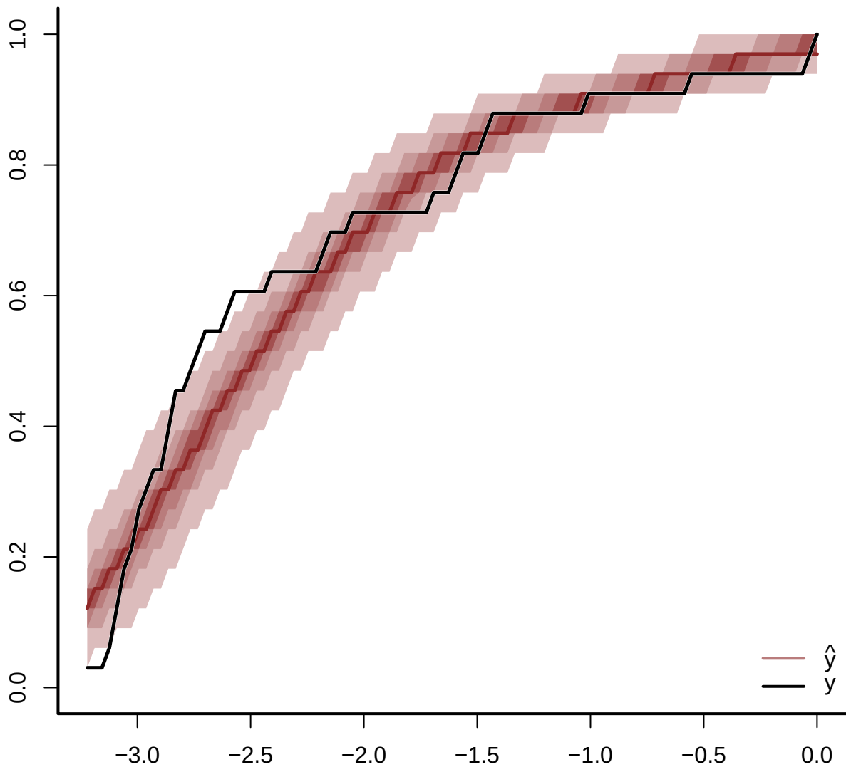
Predictive CDF for SEBASTES_MENTELLA
