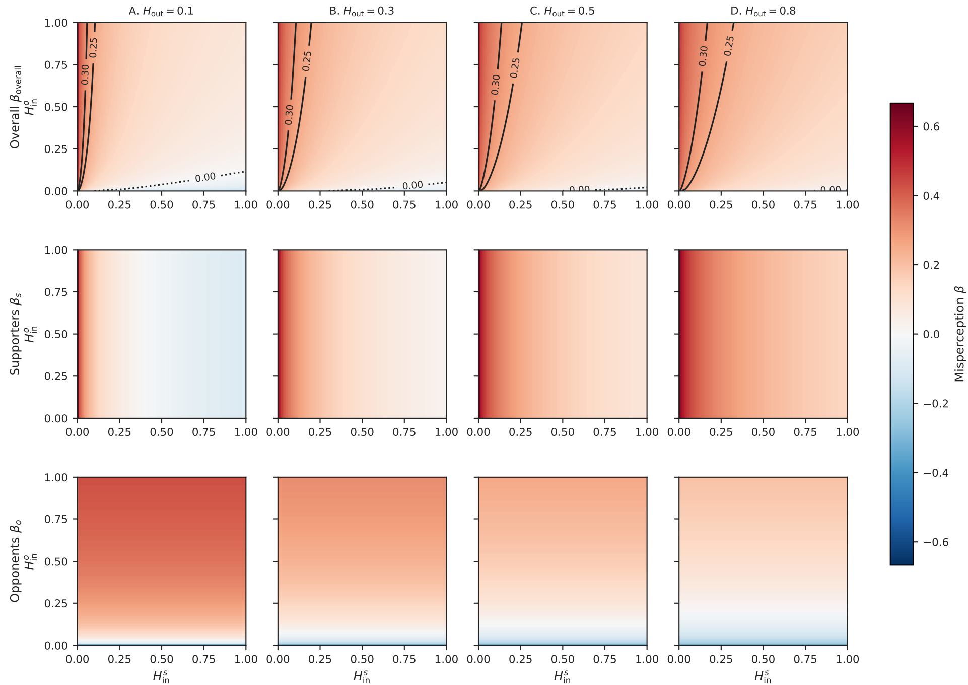
SBM misperception varying H_{\text{out}} ( \delta = 0.5 , \gamma = 0.5 )
