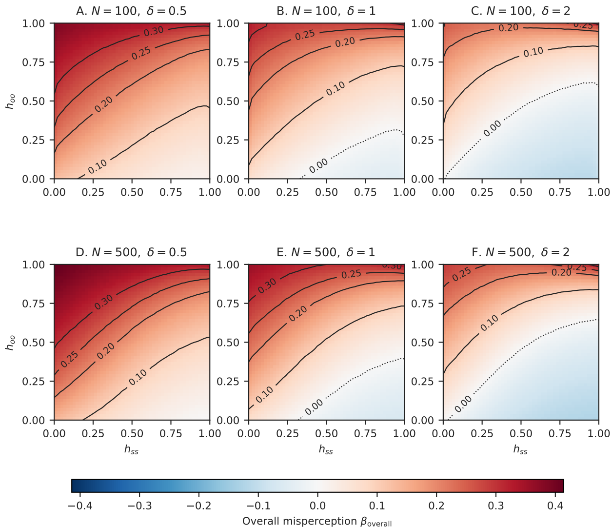
Overall misperception \beta_{\text{overall}} — varying N and \delta ( m = 5 , \gamma = 0.5 )
