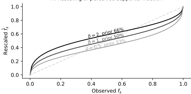
A. Rescaling of perceived supporter fraction
