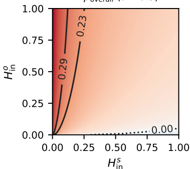
F. \beta_{\text{overall}} ( \delta = 0.5 )
