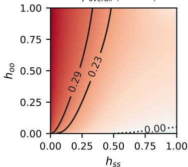
Rescaled misperception on stochastic block networks ( \gamma = 0.5 , fixed H_{\text{out}} = 0.3 )
