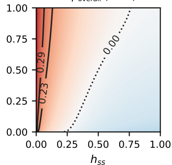
Rescaled misperception on stochastic block networks ( \gamma = 0.5 , fixed H_{\text{out}} = 0.3 )
