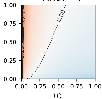
H. \beta_{\text{overall}} ( \delta = 2 )
