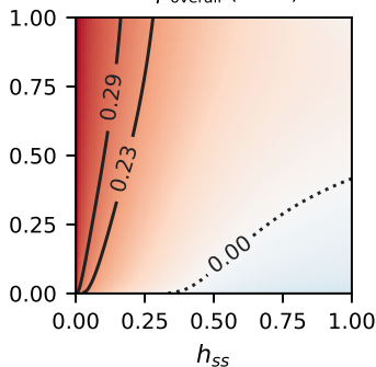
Rescaled misperception on stochastic block networks ( \gamma = 0.5 , fixed H_{\text{out}} = 0.3 )
