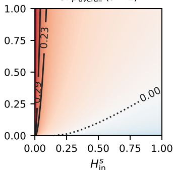
G. \beta_{\text{overall}} ( \delta = 1 )
