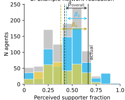
B. Example network realization
