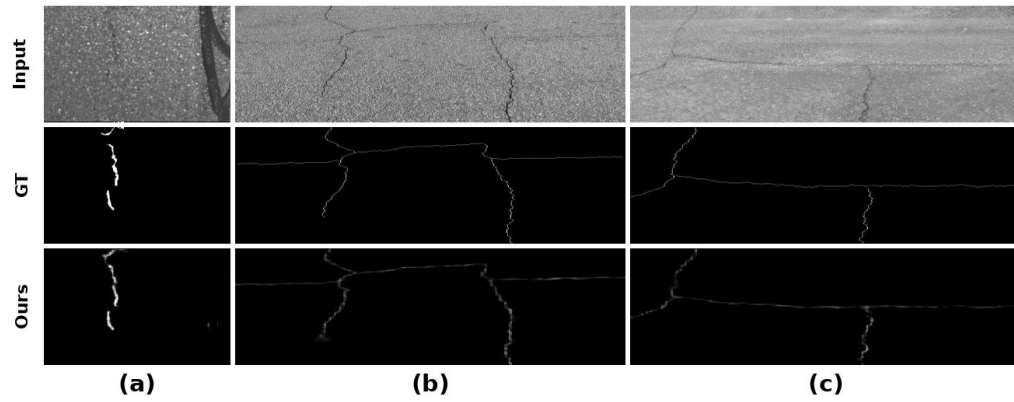
Fig. 2. Representative failure cases of FANet on the most challenging crack categories. In each column, the top row is the input image, the middle row is the ground truth, and the bottom row is our prediction. (a) A camouflaged, low-contrast crack whose connected ground-truth structure is fragmented into disconnected segments by our prediction. (b), (c) Fine hairline cracks whose complete ground truth is only weakly and partially recovered by our prediction.
