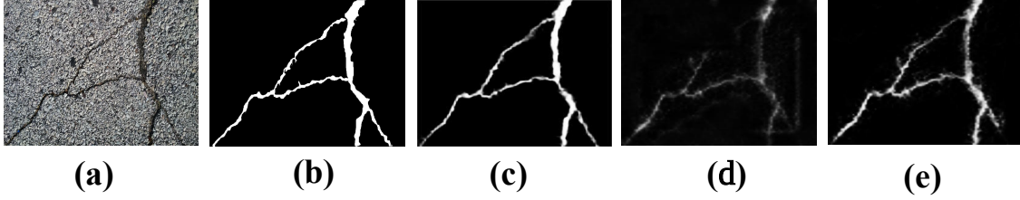
Fig. 1. Qualitative comparison of the three FAM configurations in Table II on a typical sample selected from the test set as an illustrative case. (a) Input. (b) Ground truth. (c) Prediction of FAM (Full) , which fuses the high- and low-frequency branches, per-sample IoU = 0.79 . (d) Prediction of FAM (High-Freq only) , per-sample IoU = 0.61 . (e) Prediction of FAM (Low-Freq only) , per-sample IoU = 0.57 . The full-fusion configuration preserves both the main crack contour and the hairline branches, which is consistent with the quantitative gains reported in Table II.
