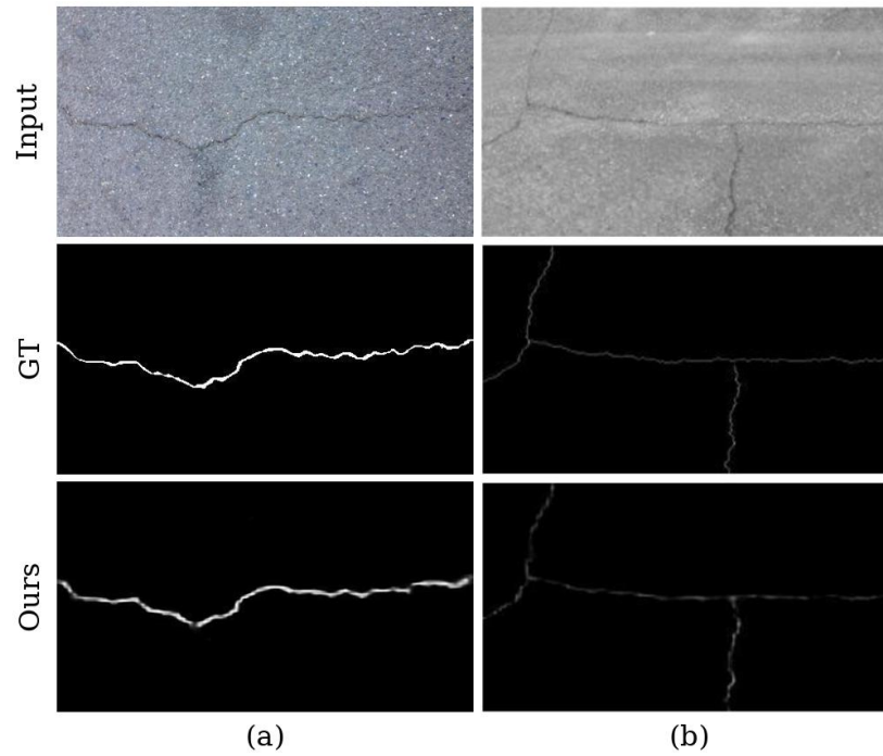
Fig. 7. Illustrative failure cases of FANet. In each column, the top, middle, and bottom rows show the input image, the ground truth, and our prediction, respectively. (a) A low-contrast crack whose continuous ground-truth structure is only weakly and unevenly recovered, losing continuity at several locations. (b) A fine hairline crack whose main structure is recovered while several fine branches are missed or only partially detected.
