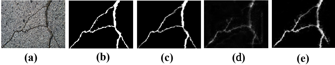
Fig. 6. Qualitative comparison of three FAM configurations in Table II on a purposefully selected illustrative case from the Crack500 test set. (a) Input. (b) Ground truth. (c) Prediction of Baseline + FAM (Full) , which fuses the high- and low-frequency branches; per-image AIU = 0.62. (d) Prediction of Baseline + FAM (High-Freq) ; per-image AIU = 0.45. (e) Prediction of Baseline + FAM (Low-Freq) ; per-image AIU = 0.41. This illustrative example qualitatively shows the complementary behavior of the two frequency branches; dataset-level conclusions are based on Table II.
