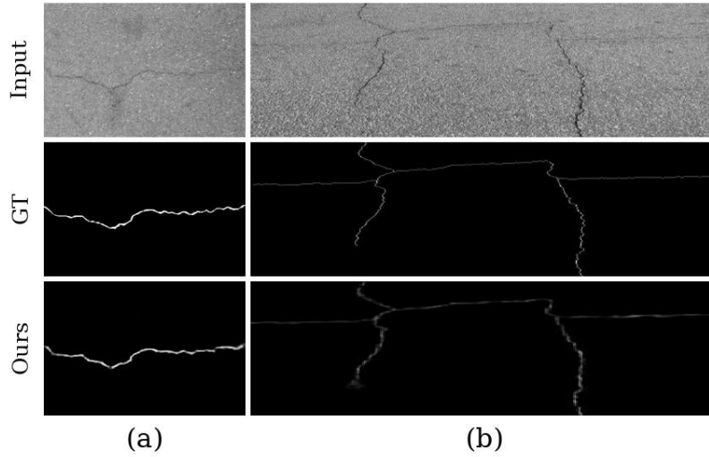
Fig. 7. Illustrative failure cases of FANet. In each column, the top, middle, and bottom rows show the input image, the ground truth, and our prediction, respectively. (a) A low-contrast crack whose continuous ground-truth structure is only weakly and unevenly recovered, losing continuity at several locations. (b) A fine hairline crack whose main structure is recovered while several fine branches are missed or only partially detected. Dataset and sample ID: [[TO FILL dataset + sample ID for (a) and (b)]].
