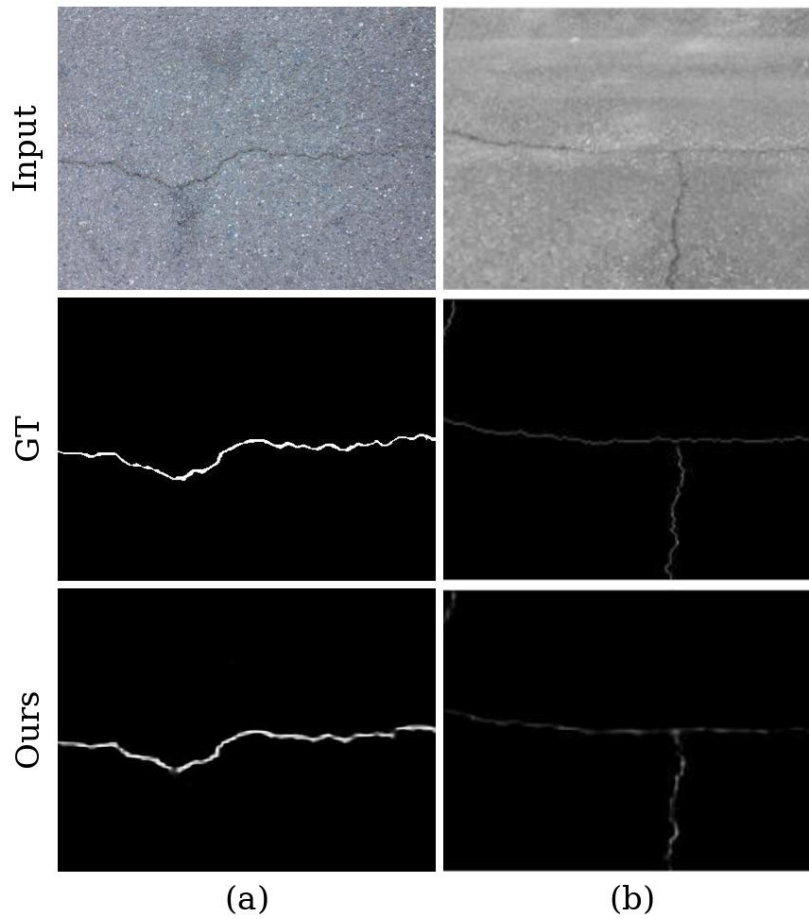
Fig. 7. Illustrative failure cases of FANet. In each column, the top, middle, and bottom rows show the input image, the ground truth, and our prediction, respectively. (a) A low-contrast crack whose continuous ground-truth structure is only weakly and unevenly recovered, losing continuity at several locations. (b) A fine hairline crack whose main structure is recovered while several fine branches are missed or only partially detected.
