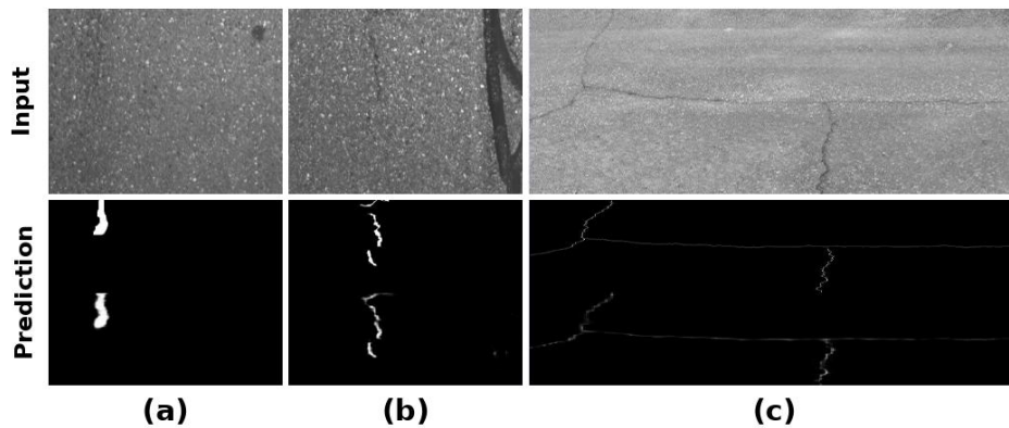
Fig. 2. Representative failure cases of FANet, taken from its own predictions on the hardest crack categories. In each column the top is the input image and the bottom is the predicted crack map. (a) A camouflaged crack is fragmented into two disconnected blobs; (b) a low-contrast crack is broken into short segments; (c) fine hairline cracks are weakly activated and partly missed.
