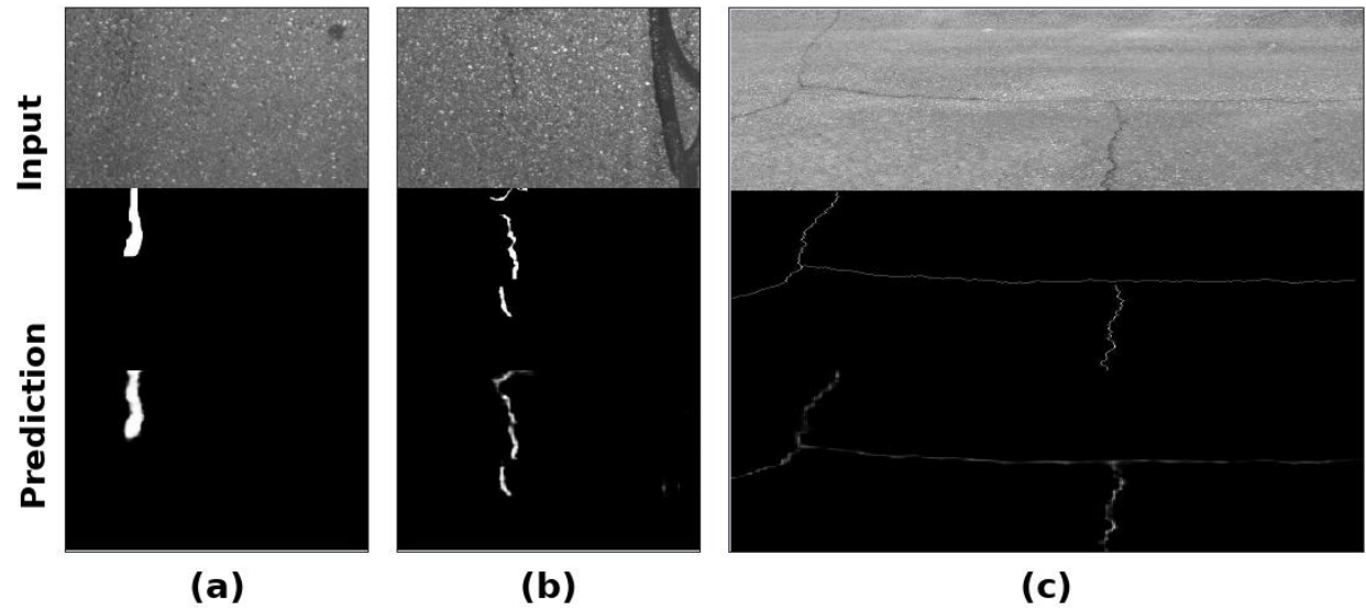
Fig. 2. Representative failure cases of FANet, taken from its own predictions on the hardest crack categories. In each column the top is the input image and the bottom is the predicted crack map. (a) A camouflaged crack is fragmented into two disconnected blobs; (b) a low-contrast crack is broken into short segments; (c) fine hairline cracks are weakly activated and partly missed.
