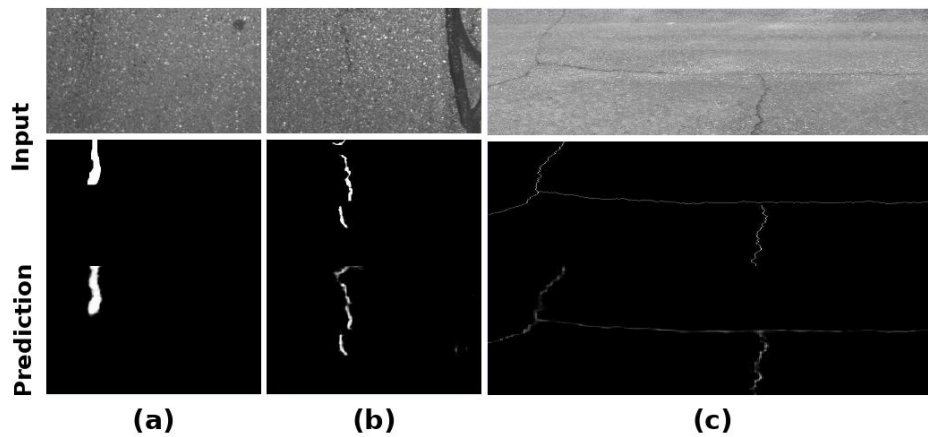
Fig. 2. Representative failure cases of FANet, taken from its own predictions on the hardest crack categories. In each column the top is the input image and the bottom is the predicted crack map. (a) A camouflaged crack is fragmented into two disconnected blobs; (b) a low-contrast crack is broken into short segments; (c) fine hairline cracks are weakly activated and partly missed.
