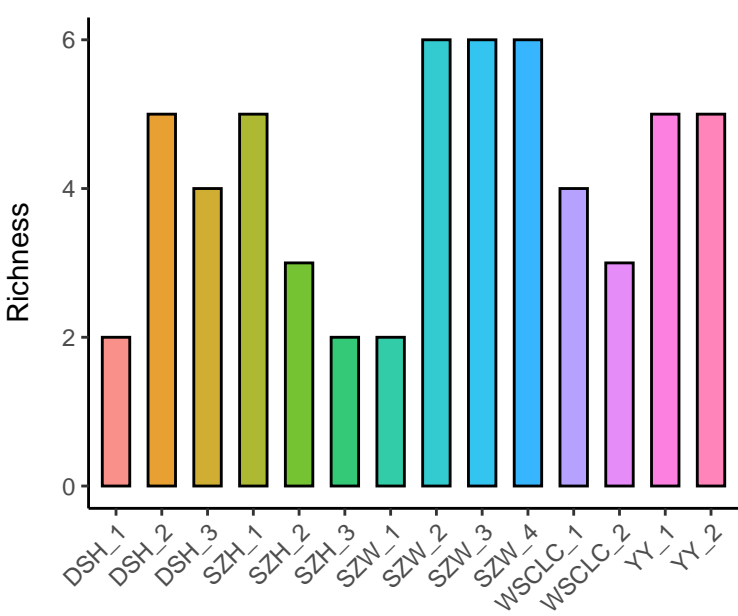
Richness Index
