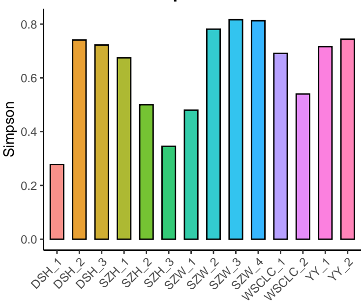
Simpson Index
