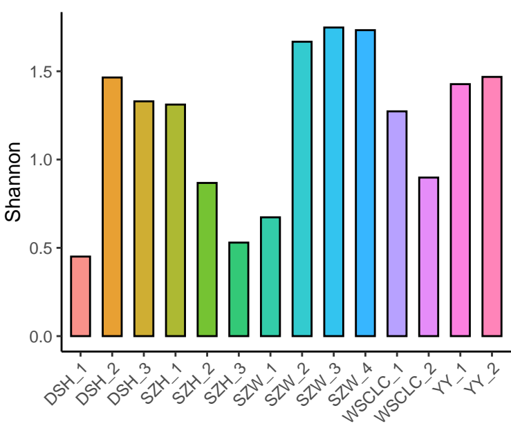
Shannon Index
