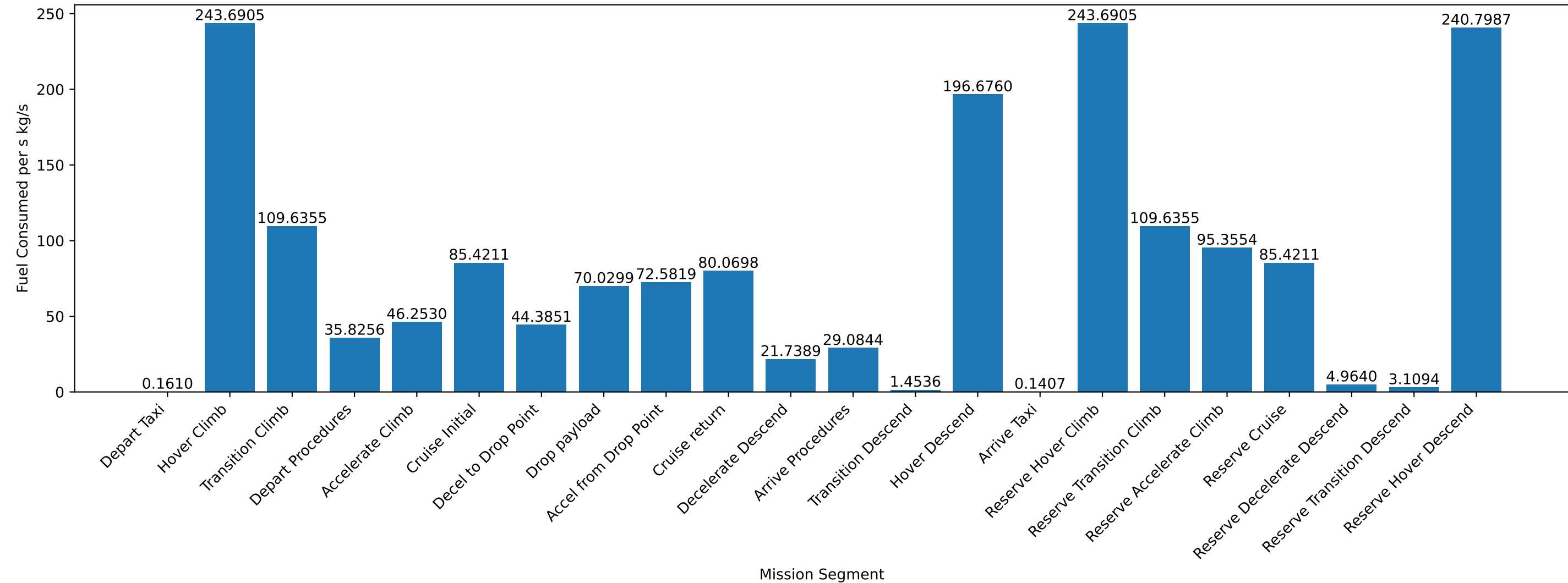
Mission Segment Fuel Consumption
