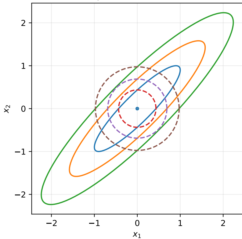
\rho = 0.9, \kappa = 19.0
