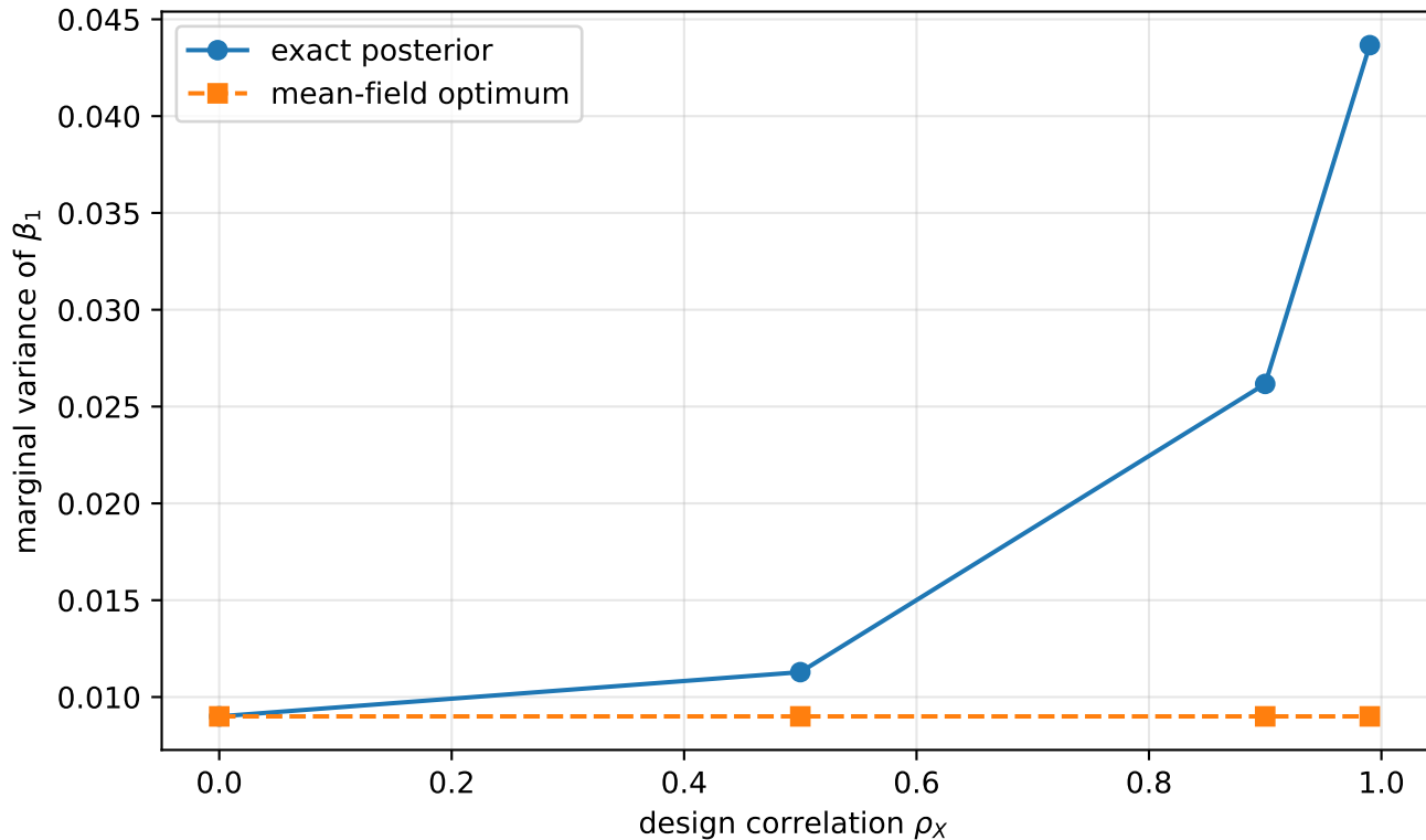
Posterior vs mean-field variance, \tau = 0.3
