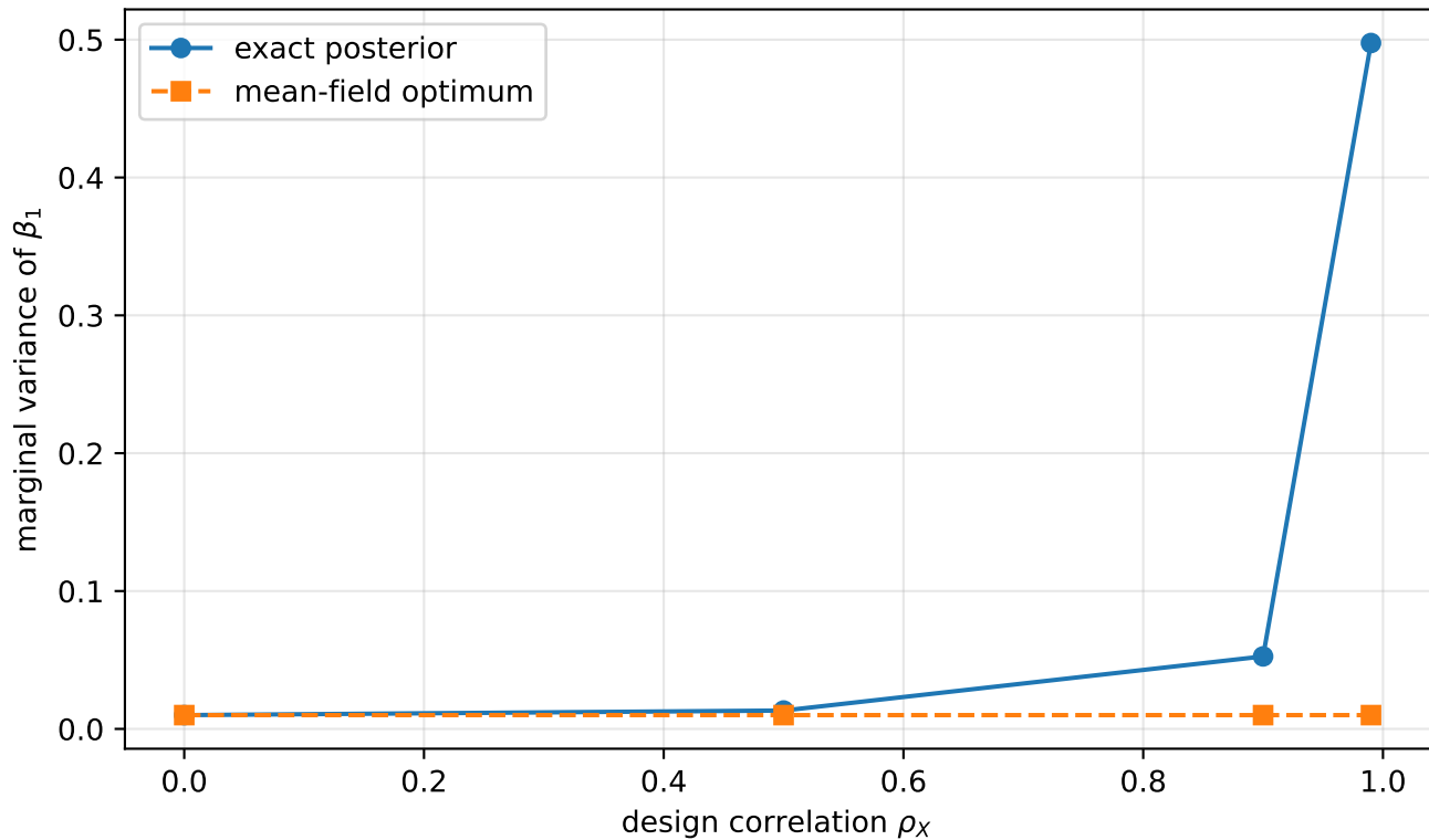
Posterior vs mean-field variance, \tau = 10
