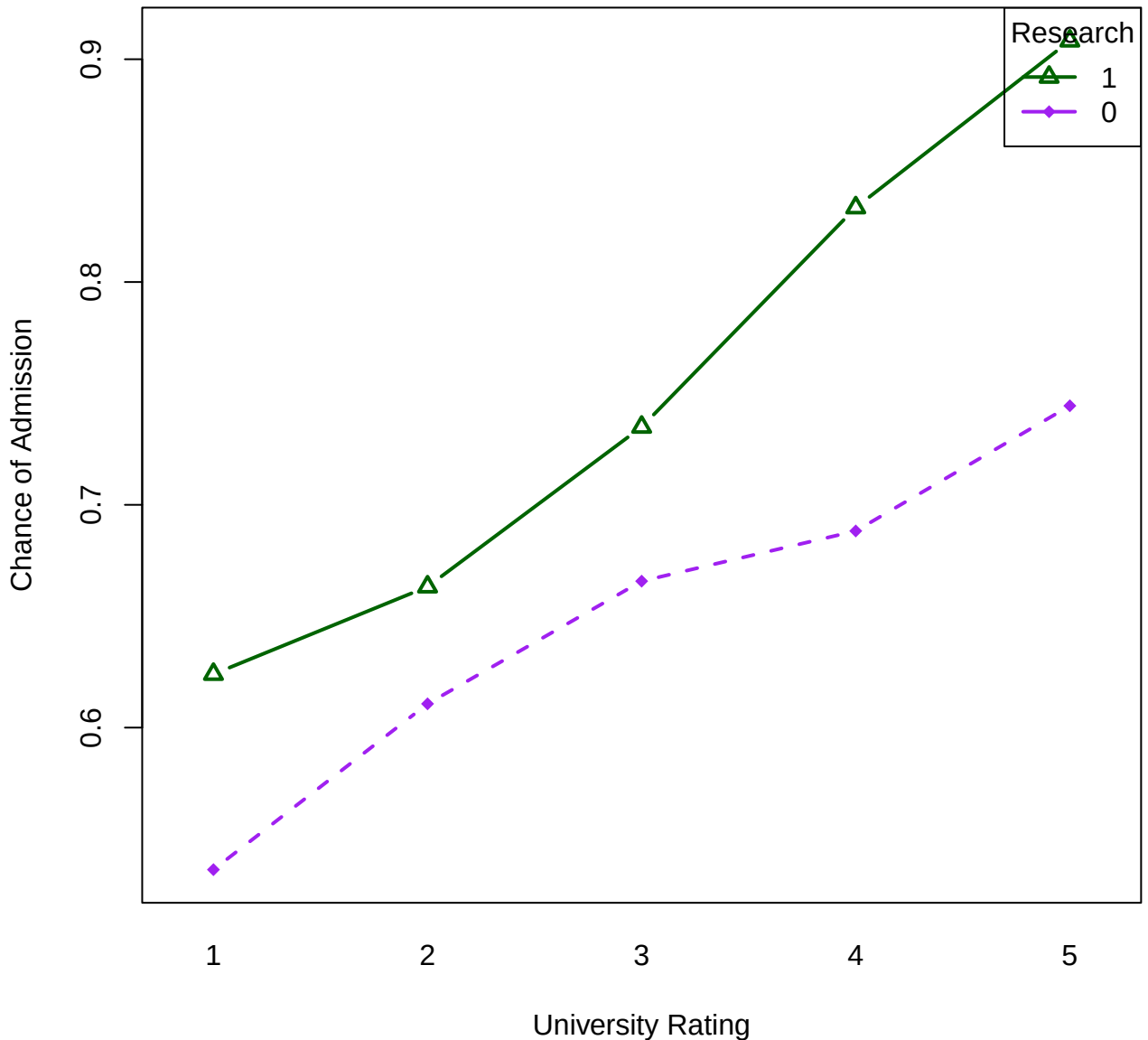
Interaction Plot
