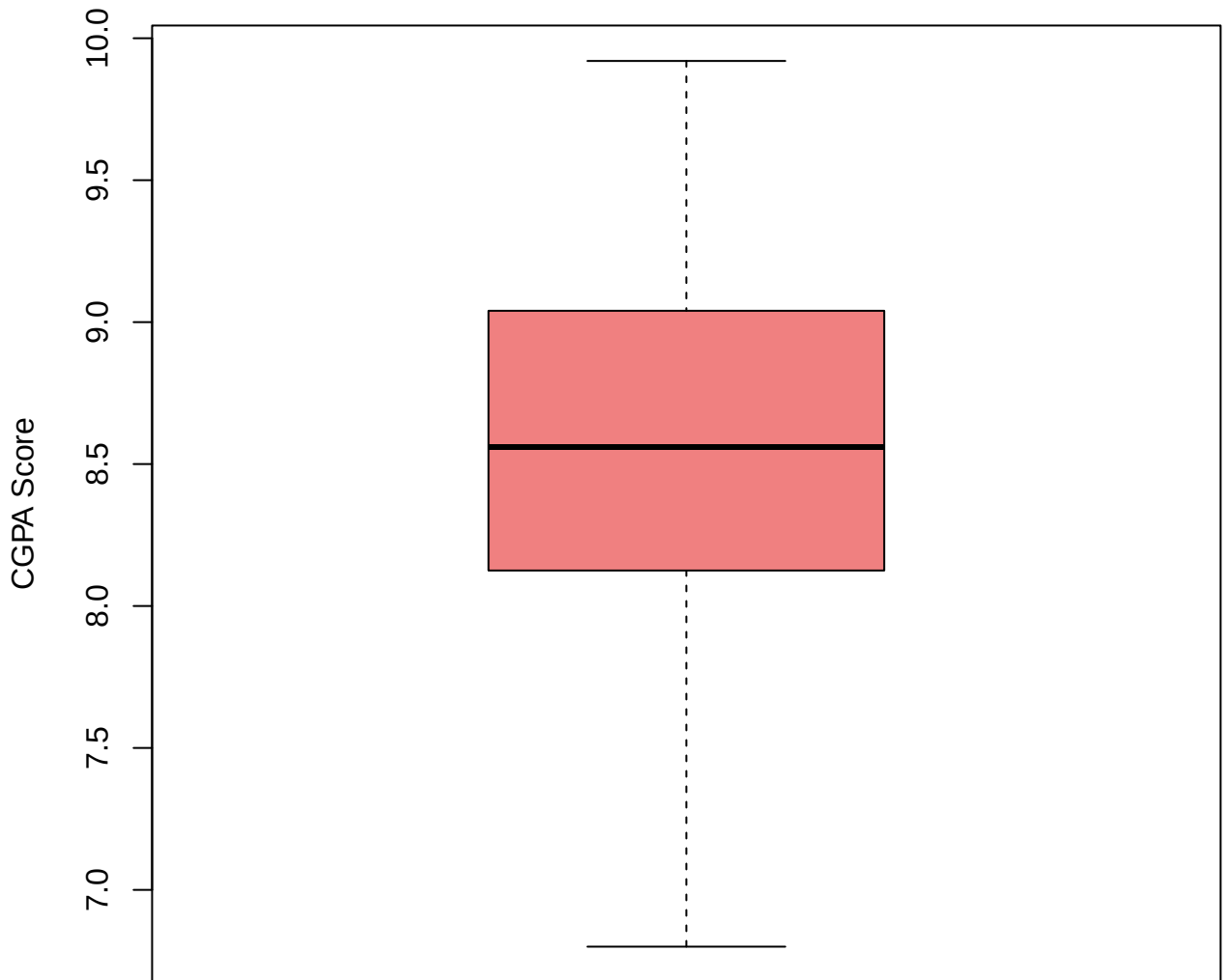
Boxplot for CGPA Scores
