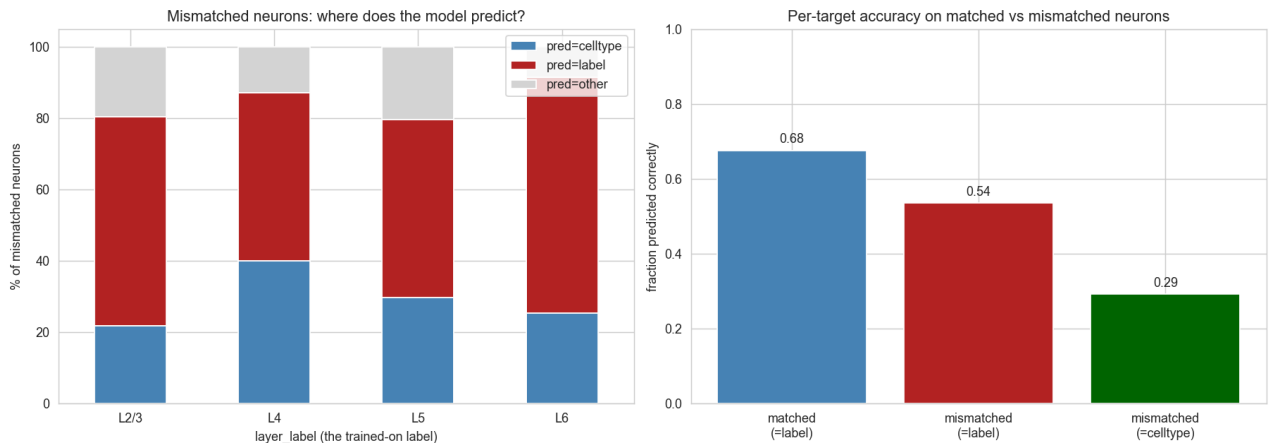
Figure 3: Where the model predicts for mismatched neurons. Left: stacked bars show, for each layer, the fraction of mismatched neurons whose predicted label matches the depth-derived label (red), the cell-type label (blue), or neither (grey). Red dominates in every layer, indicating that the model consistently follows the depth-derived label rather than the cell-type label. Right: prediction accuracy for three groups: matched neurons scored against their depth label (0.68), mismatched neurons scored against their depth label (0.54), and mismatched neurons scored against their cell-type label (0.29). Accuracy is lower for mismatched neurons under either scoring, and lowest when scored against the cell-type label, consistent with these neurons being genuine boundary cases rather than systematic annotation errors.
