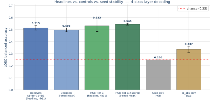
Figure 1: Oracle fingerprint vs. confound baselines. Tier G HGB (z-scored, 5-seed mean) reaches 0.545 LOSO balanced accuracy, well above the scan-only baseline (0.25, at chance) and the cc_abs -only response-quality baseline (0.337). The DeepSets A1+B+C1+D1 tabular headline (0.515) is shown for comparison.
