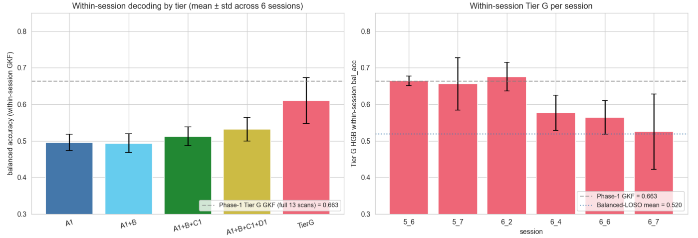
Figure 5: Within-session results. Left: within-session decoding by feature tier (mean \pm std across the well-behaved sessions). Right: Tier G HGB within-session balanced accuracy per session, against the Phase-1 GKF ceiling and the balanced-LOSO mean.
