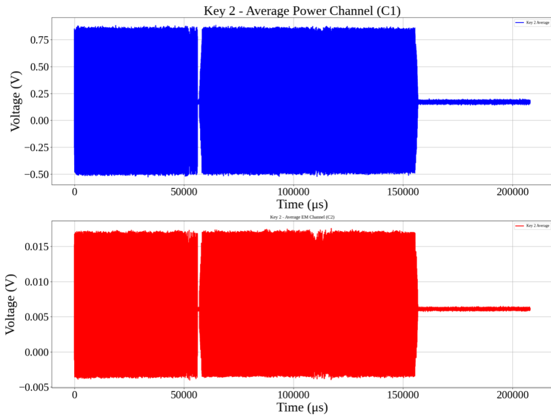
Figure 2: The Average of Key 2's Power and EM Signals
