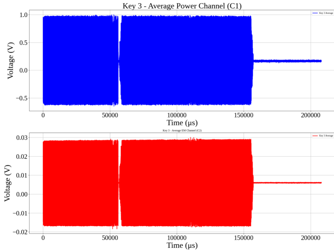
Figure 3: The Average of Key 3's Power and EM Signals
