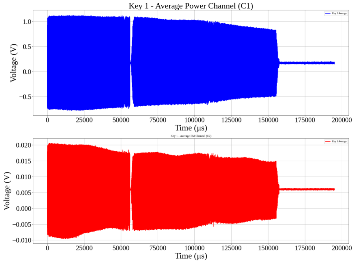
Figure 1: The Average of Key 1's Power and EM Signals
