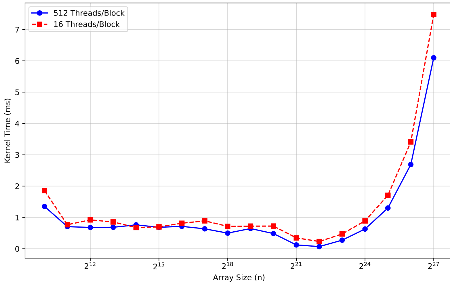
Scaling Analysis: 16 vs 512 Threads per Block
