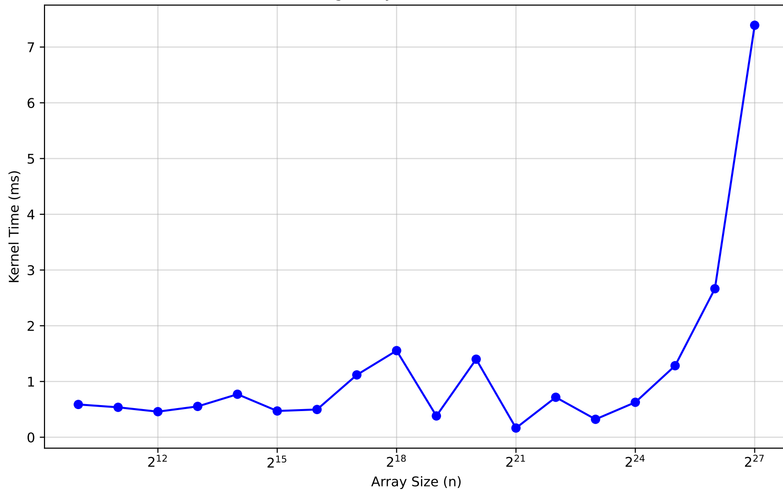
Scaling Analysis of vscale Kernel
