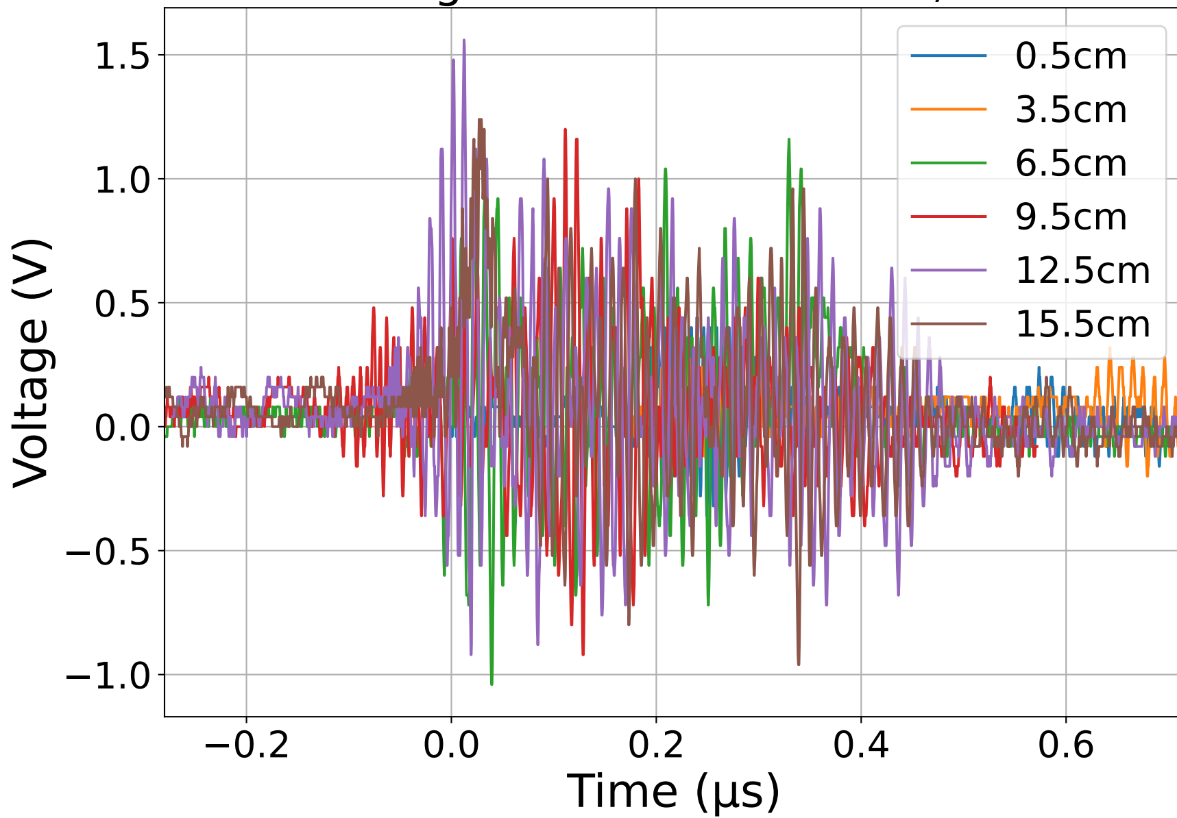
Voltage vs Time at 10.5 kV, M1
