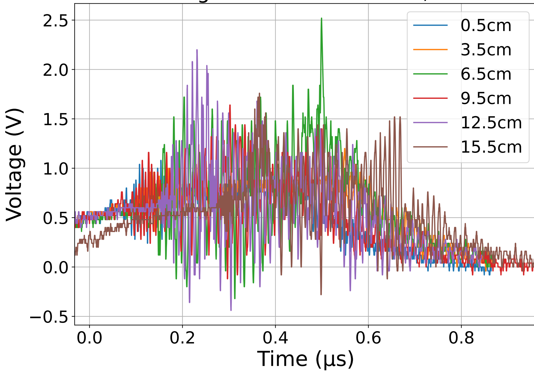
Voltage vs Time at 10.5 kV, M4
