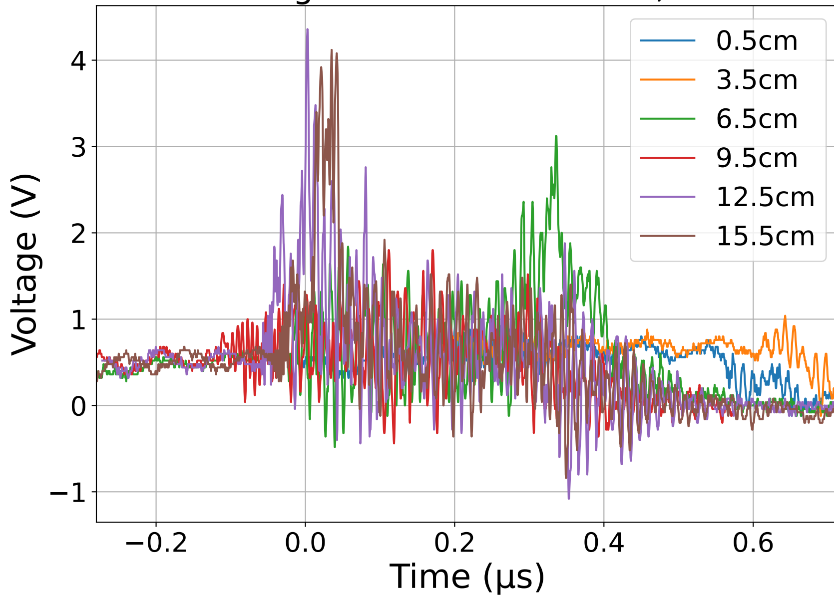
Voltage vs Time at 10.5 kV, M5
