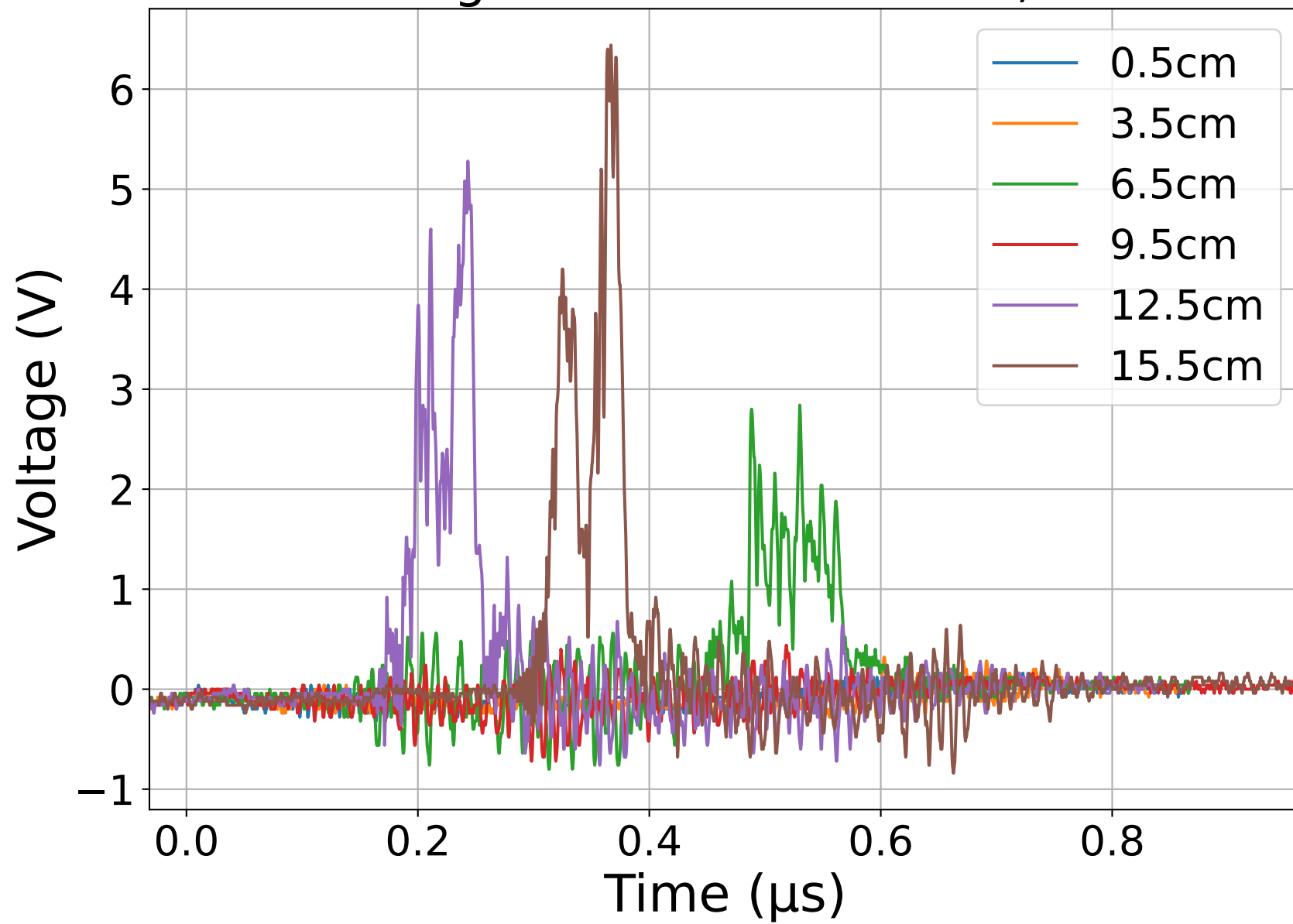
Voltage vs Time at 10.5 kV, M7
