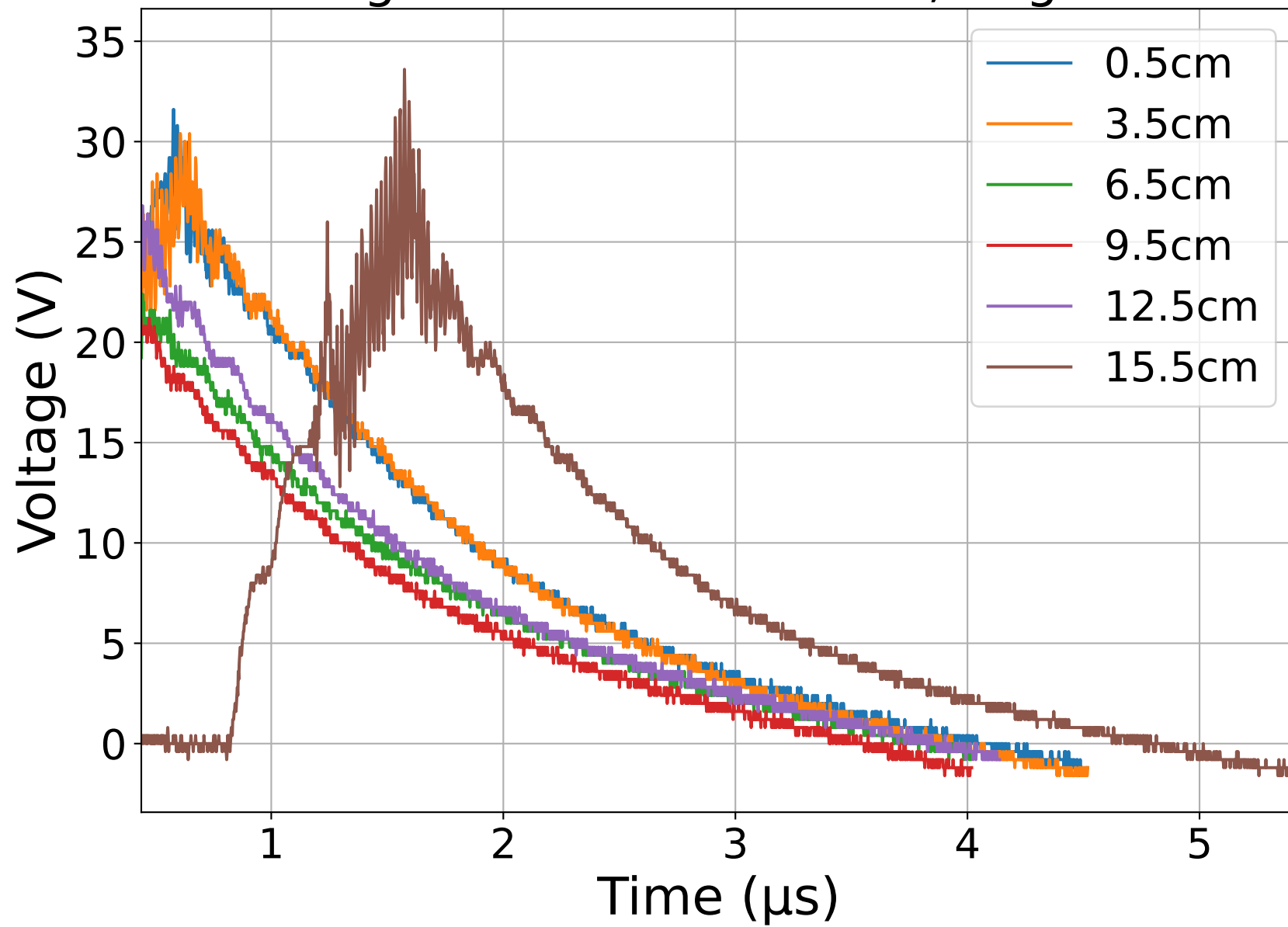
Voltage vs Time at 10.5 kV, Rogowski
