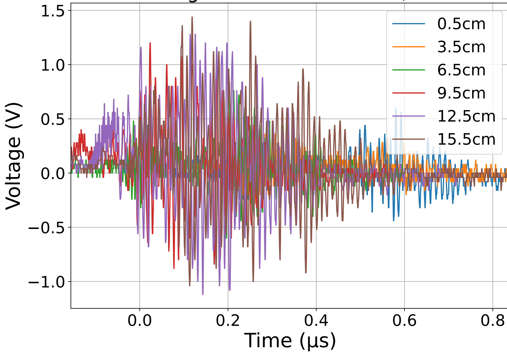
Voltage vs Time at 12.0 kV, M1
