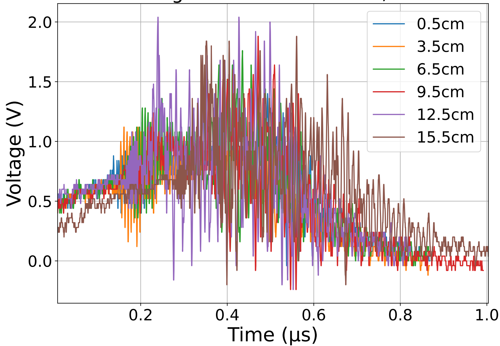
Voltage vs Time at 12.0 kV, M4
