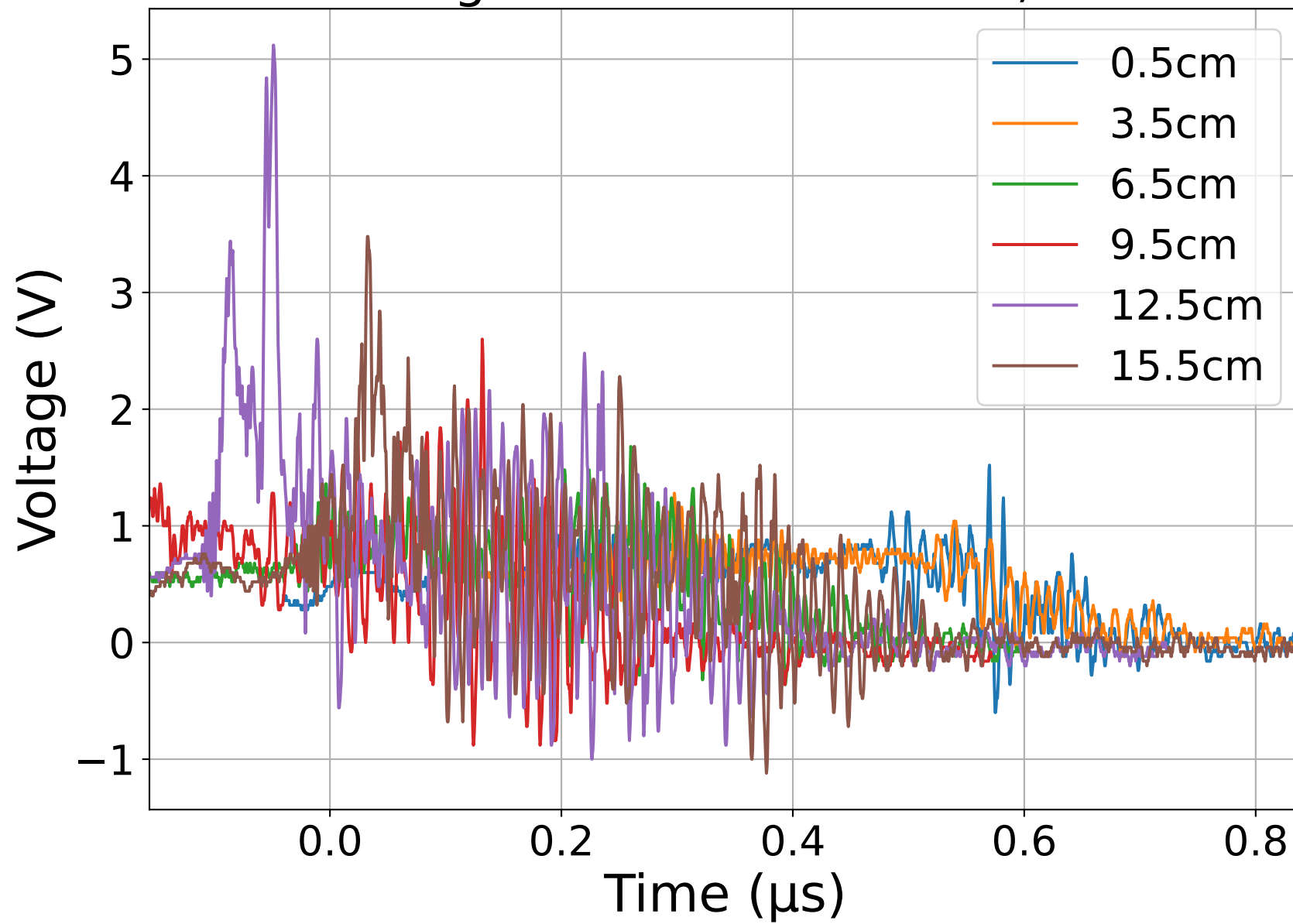
Voltage vs Time at 12.0 kV, M5
